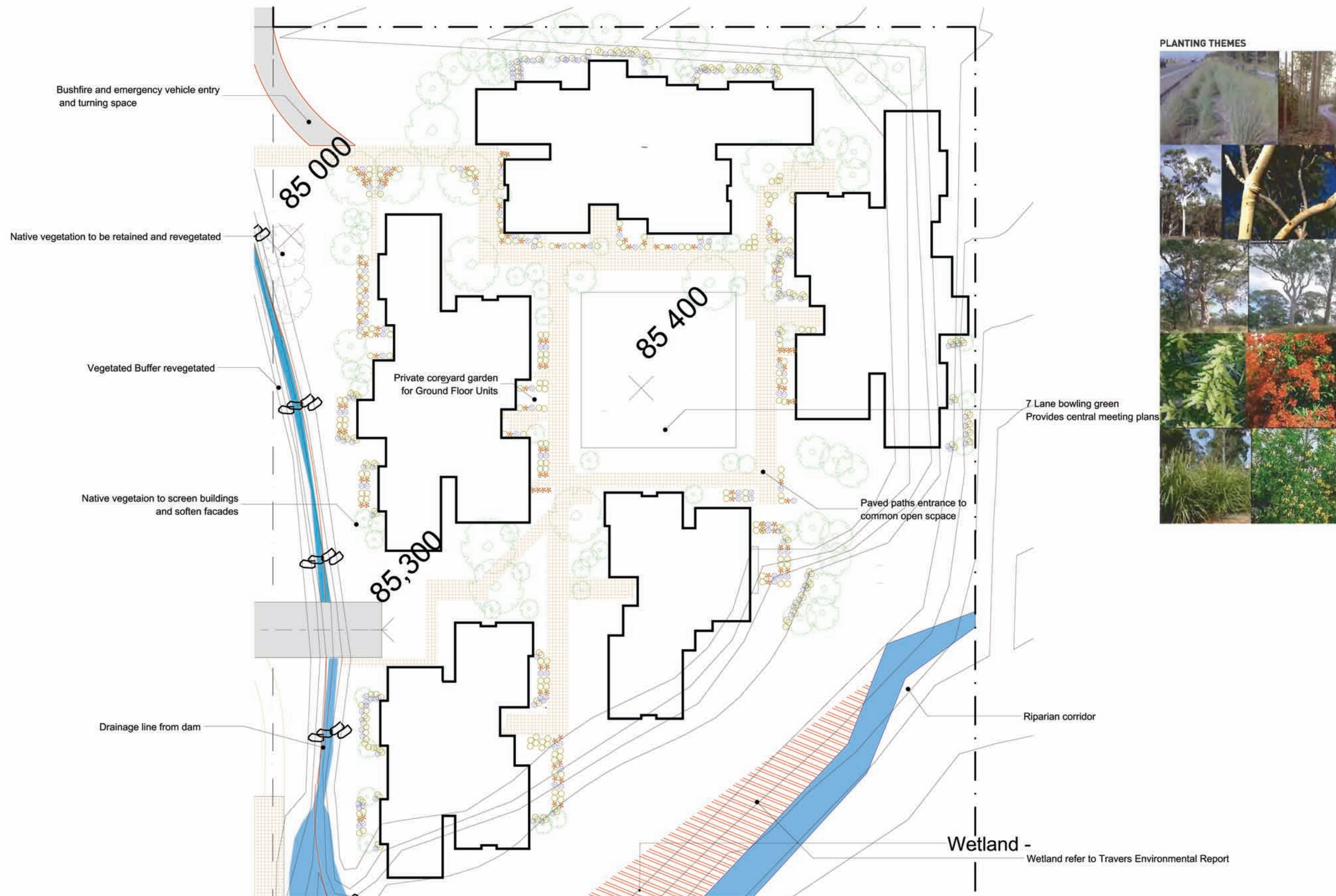
Figure 28 - Part Plan 1
