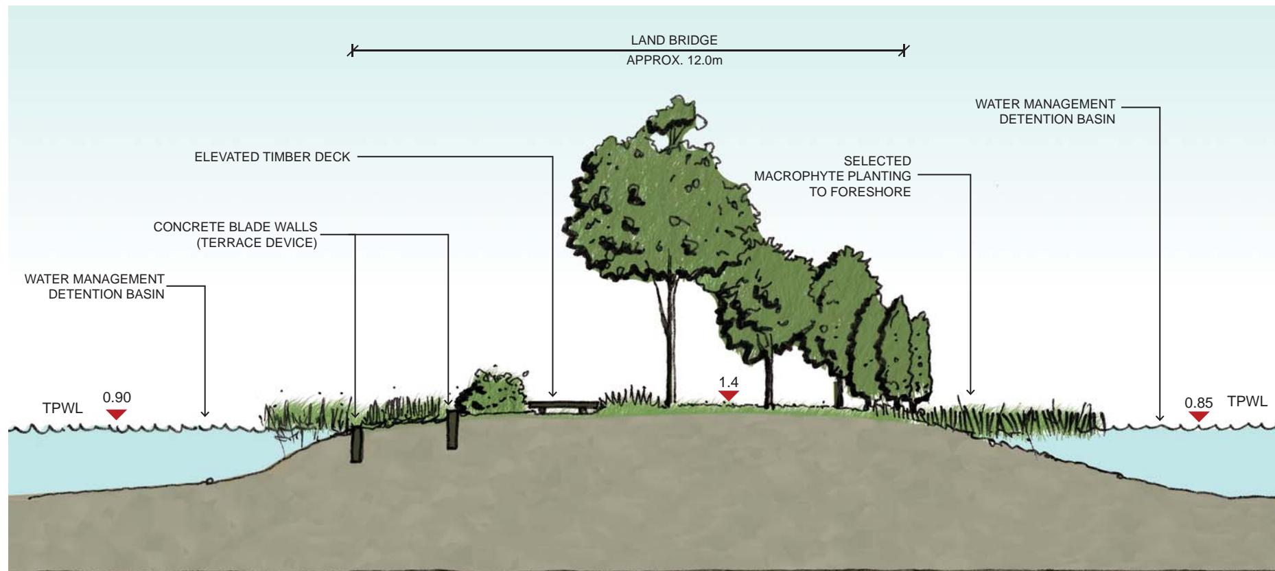
SECTION C (FROM RC-15)
