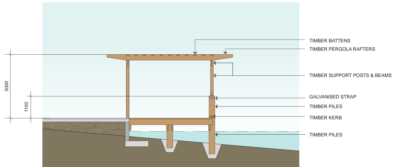
SECTION A 1
