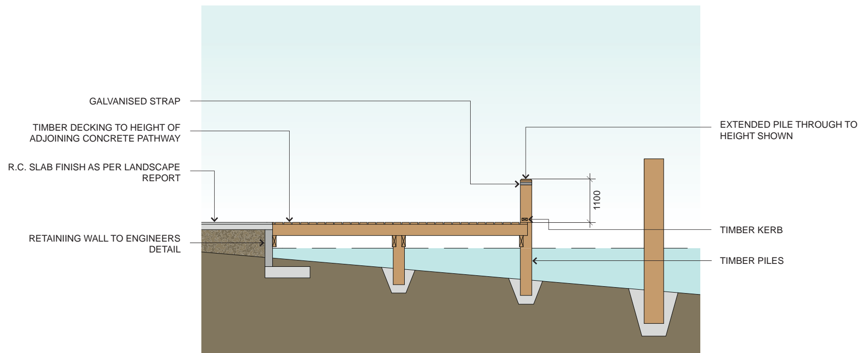
SECTION B 1
