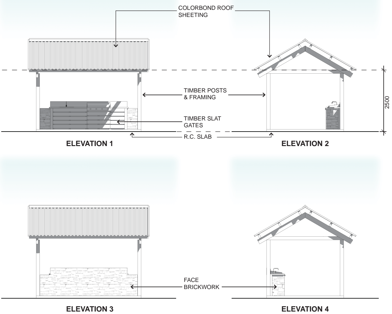
TYPICAL BBQ SHELTER
