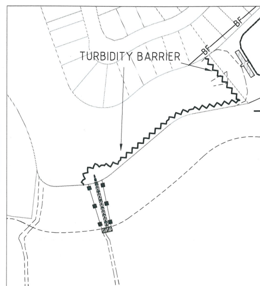
DETAIL A: SECOND OUTLET DRAIN SCALE 1:2000
