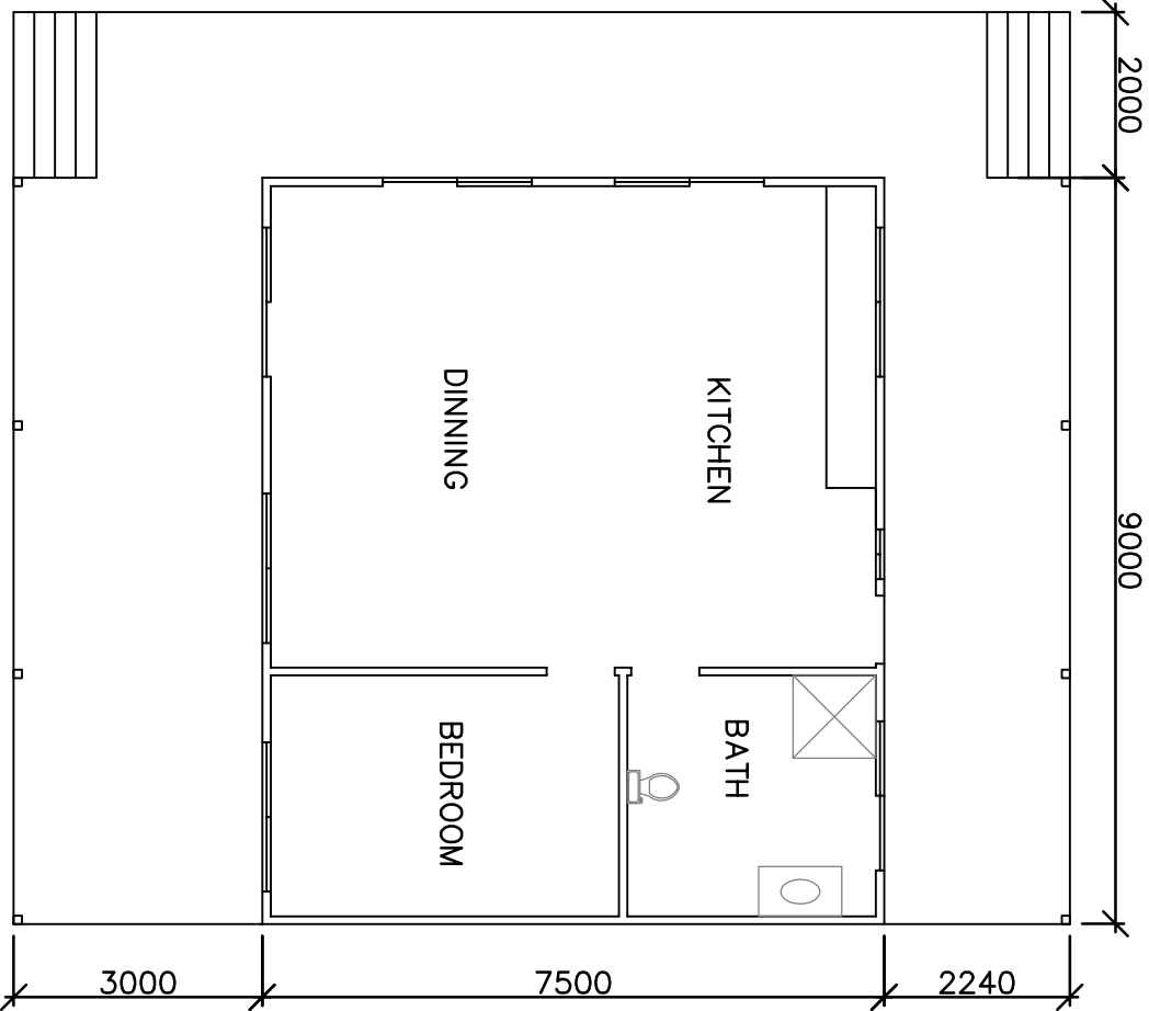
CABIN LAYOUT
