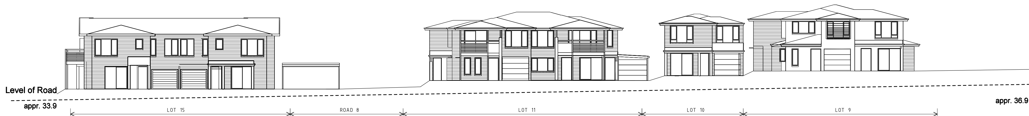
05 ELEVATION - 05 - Stage 1A - Road 4
