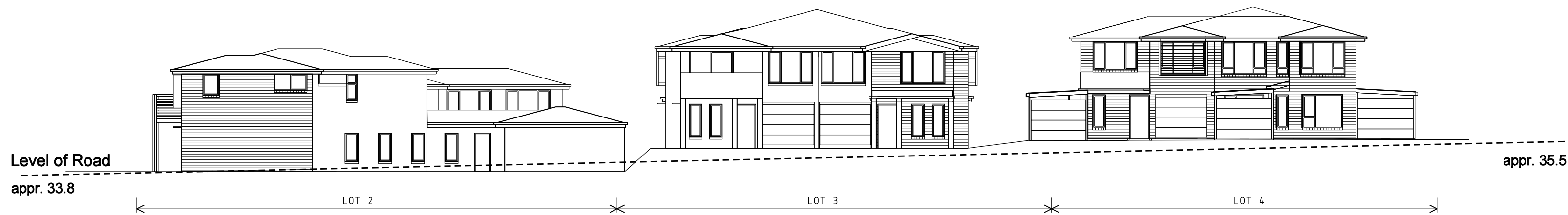
03 ELEVATION - 03 - Stage 1A - Road 3
