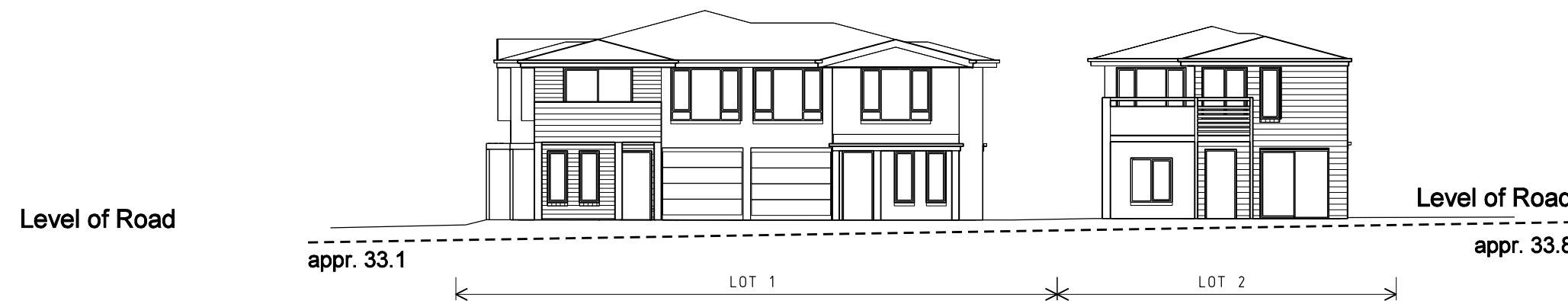
02 ELEVATION - 02 - Stage 1A - Road 1
