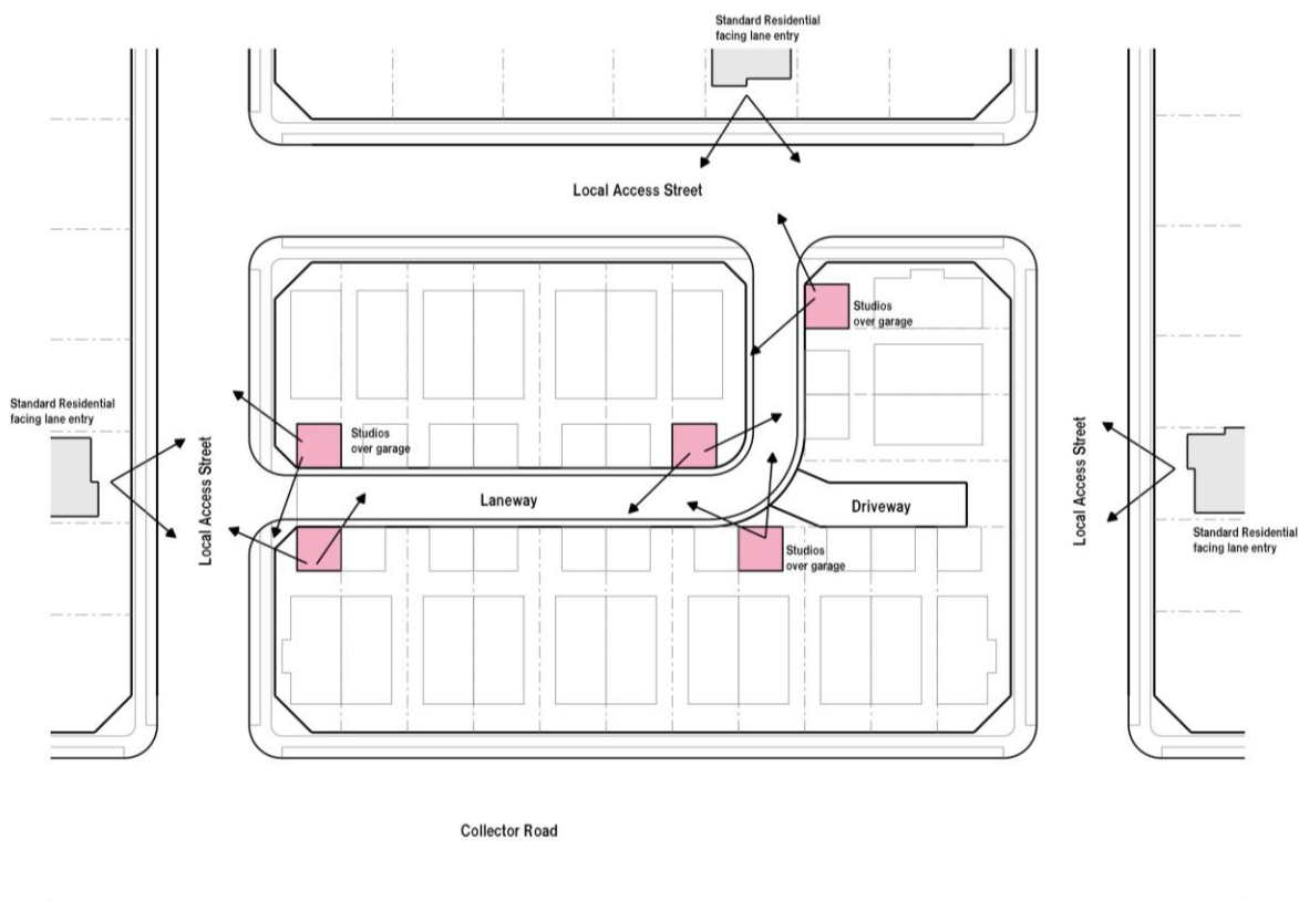
Figure 1 – Laneway Design demonstrating best practice surveillance
