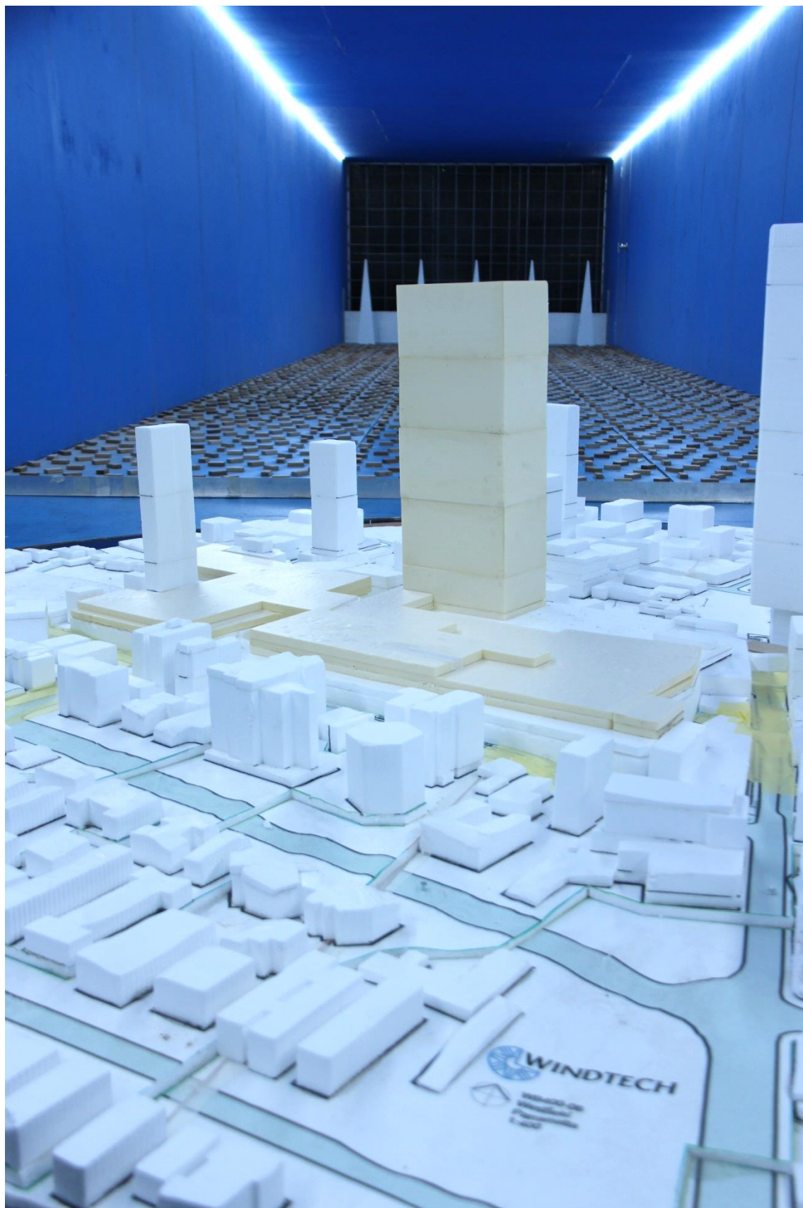
Figure 1i: Photograph of the Wind Tunnel Model – Proposed Scenario without the inclusion of the Level 6 buildings (close up view from the south-east)
