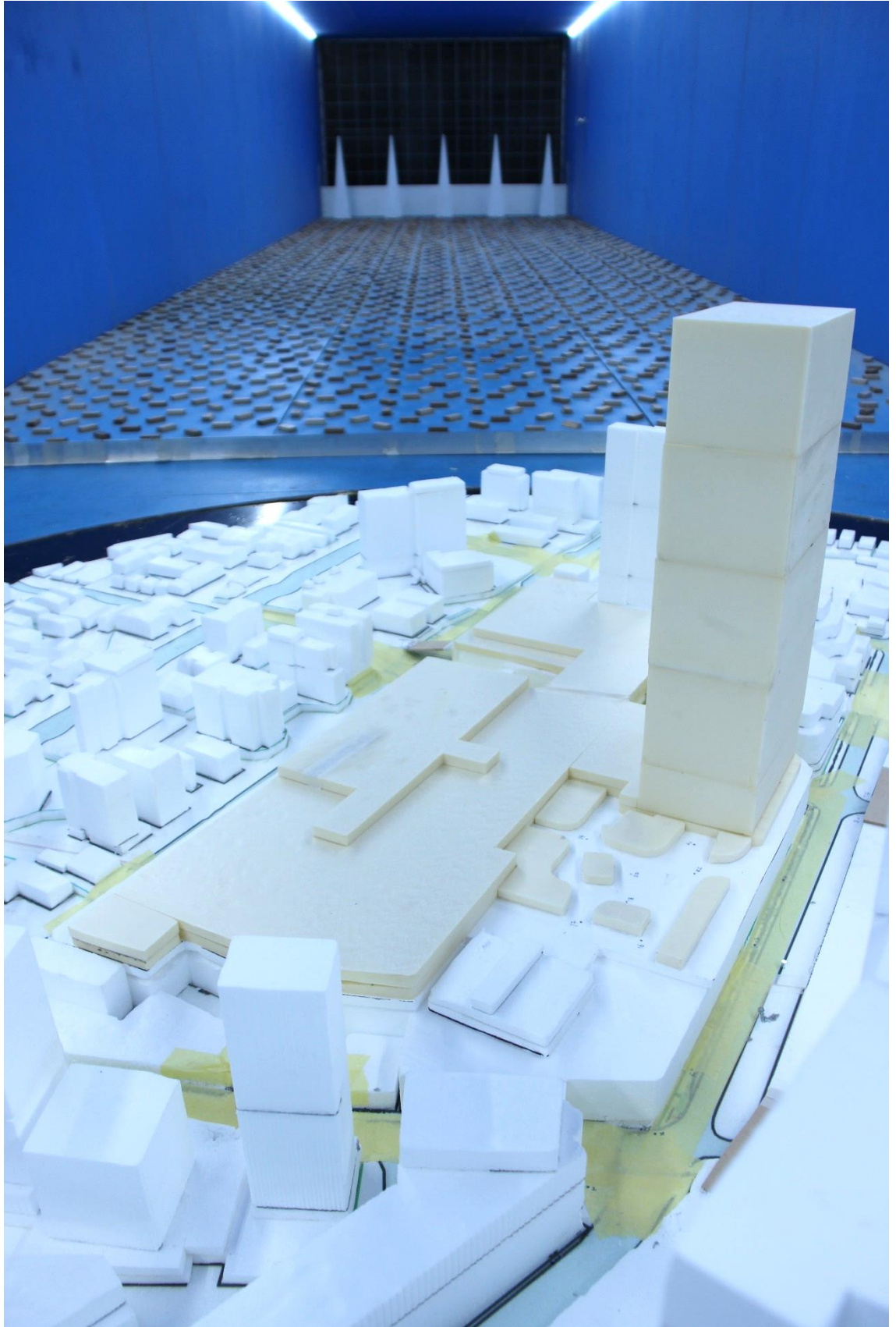
Figure 1h: Photograph of the Wind Tunnel Model – Proposed Scenario (close up view from the north-east)
