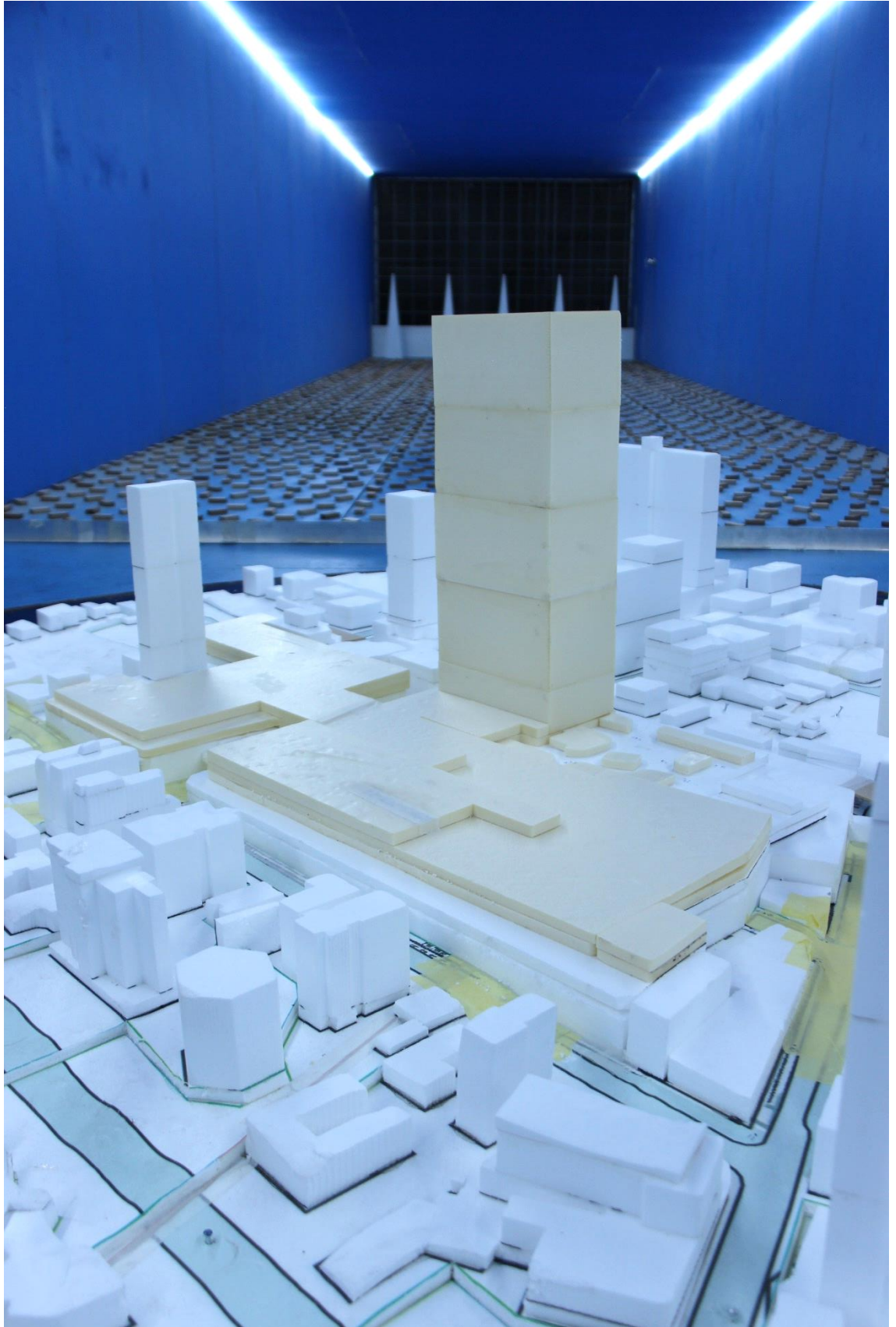
Figure 1g: Photograph of the Wind Tunnel Model – Proposed Scenario (close up view from the south-east)
