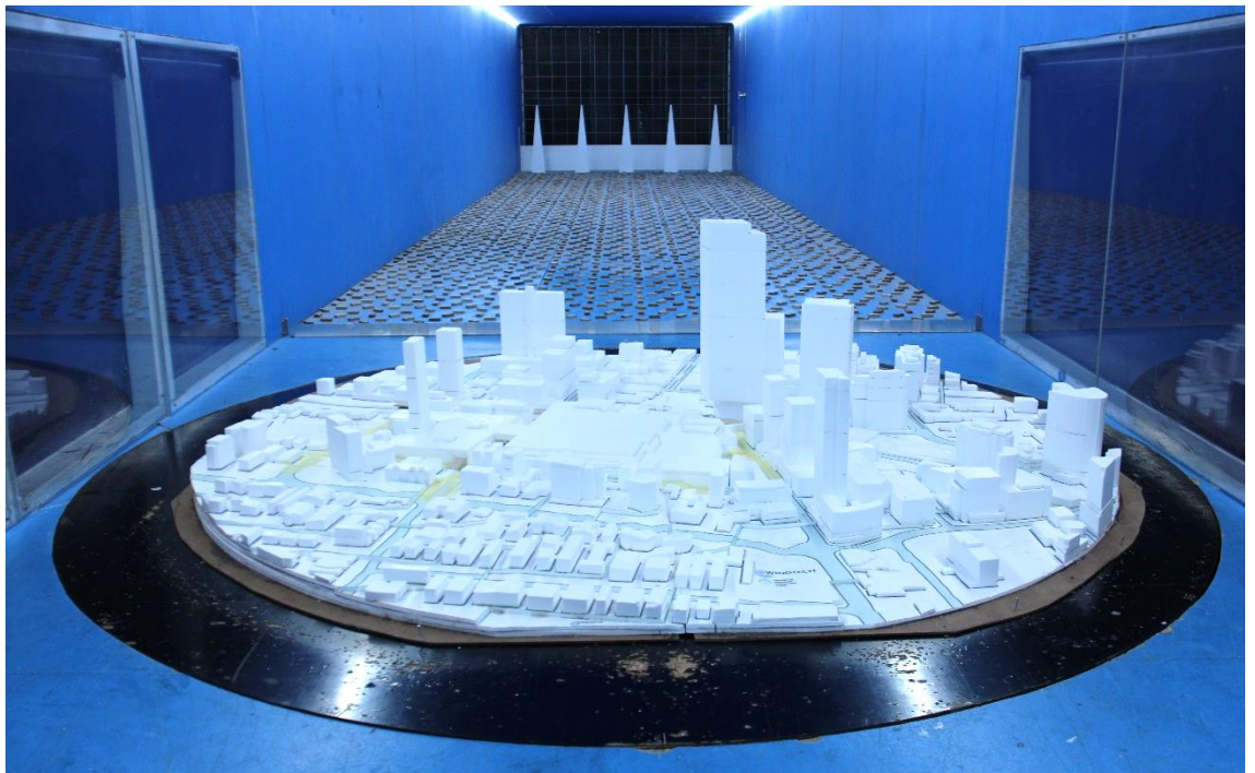
Figure 1f: Photograph of the Wind Tunnel Model – Existing Scenario (view from the south)
