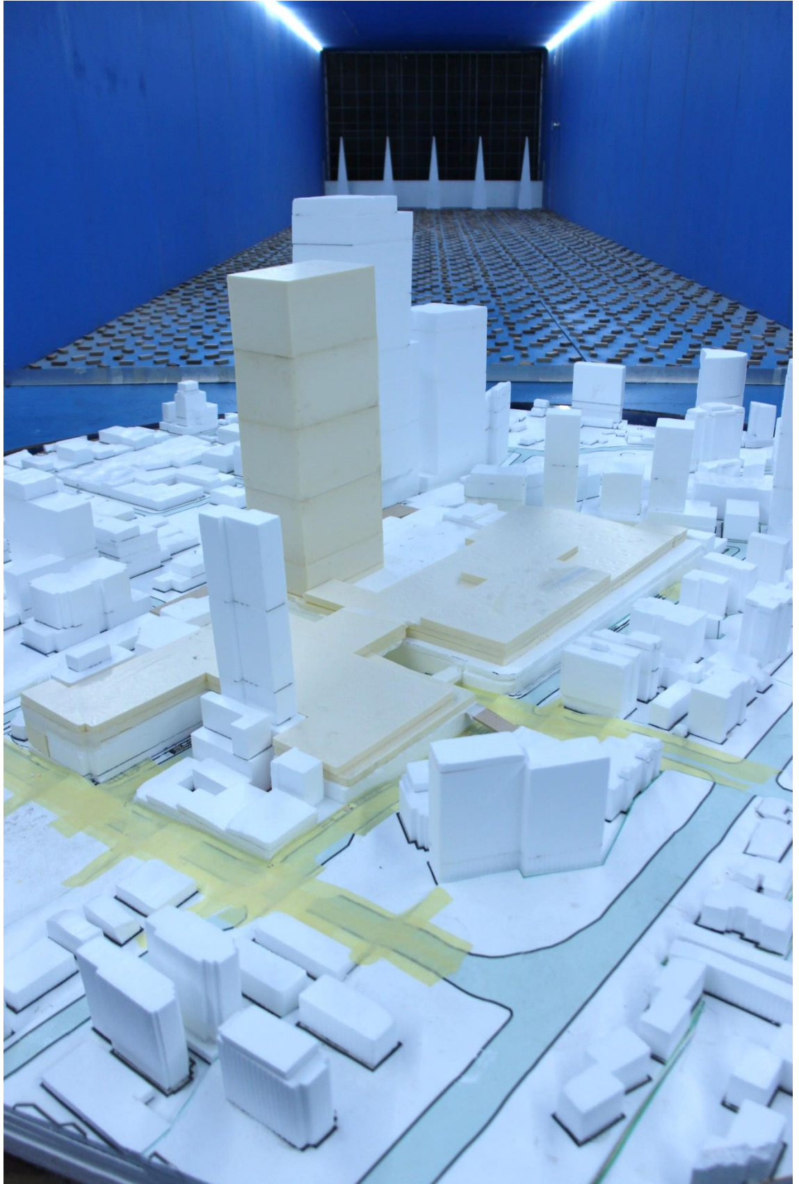
Figure 1j: Photograph of the Wind Tunnel Model – Proposed Scenario without the inclusion of the Level 6 buildings (close up view from the south-west)
