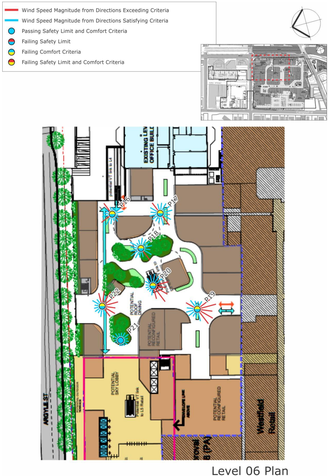
Figure 6b: Wind Tunnel Results – Level 6 Terrace Plan with the inclusion of buildings (results shown without treatments applied)
