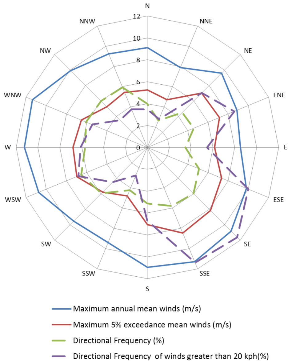
Figure 4: Annual and 5% Exceedance Hourly Mean Wind Speeds, and Frequencies of Occurrence, for the Parramatta Region (referenced to 10m above ground in standard open terrain)
