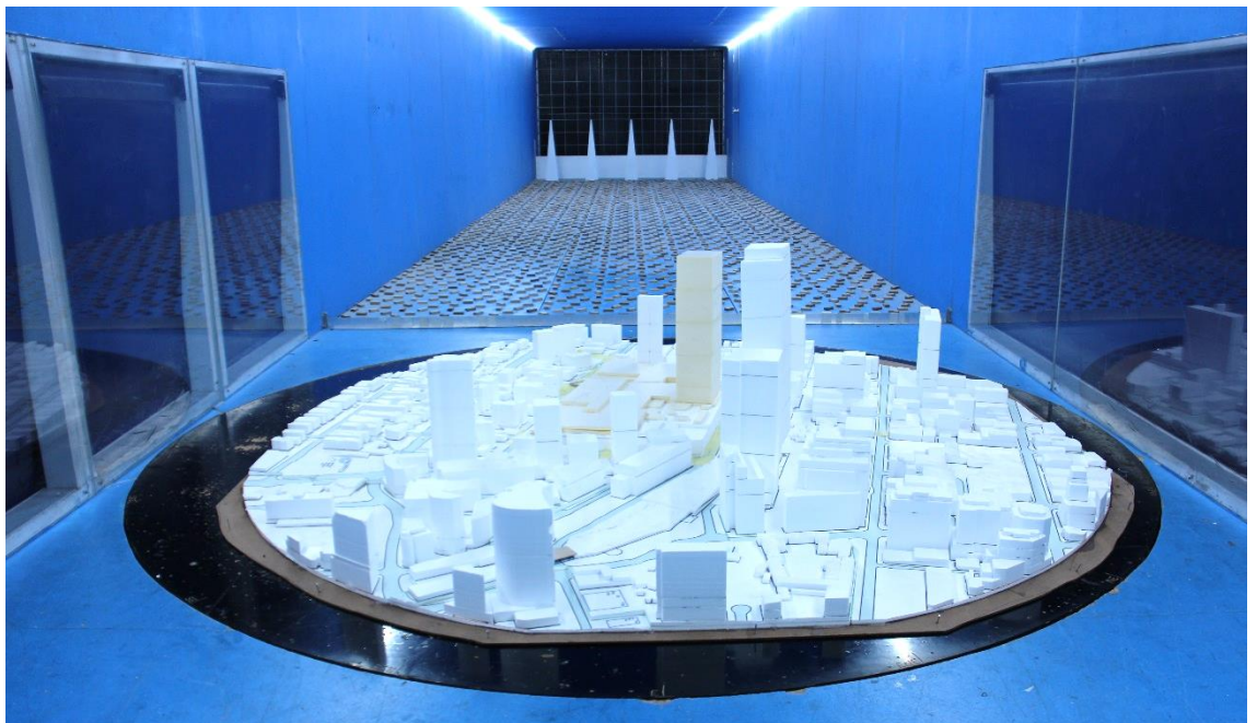
Figure 1b: Photograph of the Wind Tunnel Model – Proposed Scenario (view from the east)
