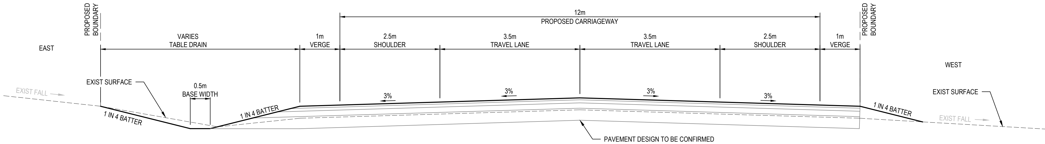
TYPICAL SECTION - TABLE DRAIN REQUIRED ON ONE SIDE SCALE 1:50
