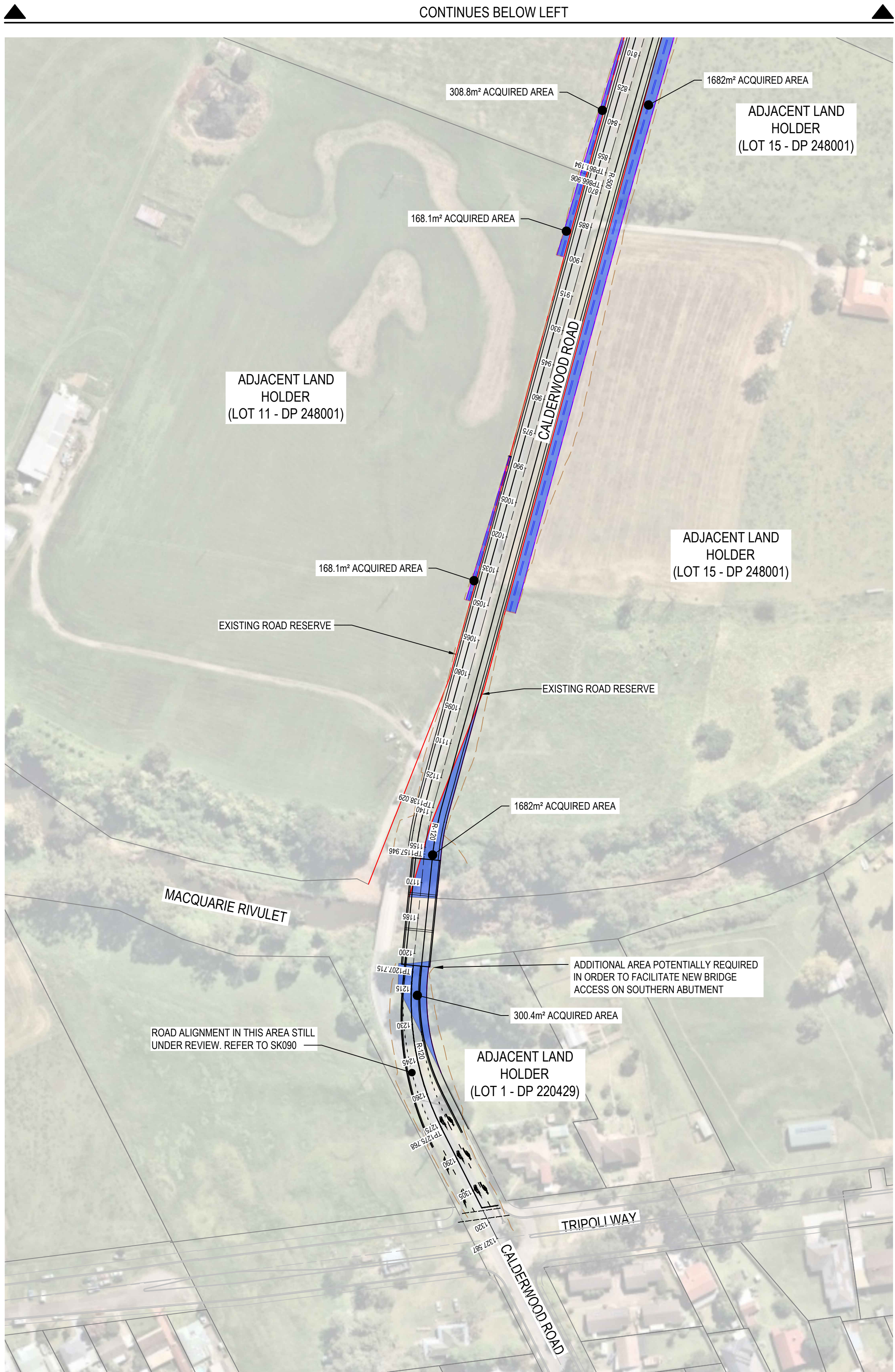
LAND ACQUISITION - CONCEPT LAYOUT SCALE 1:1250
