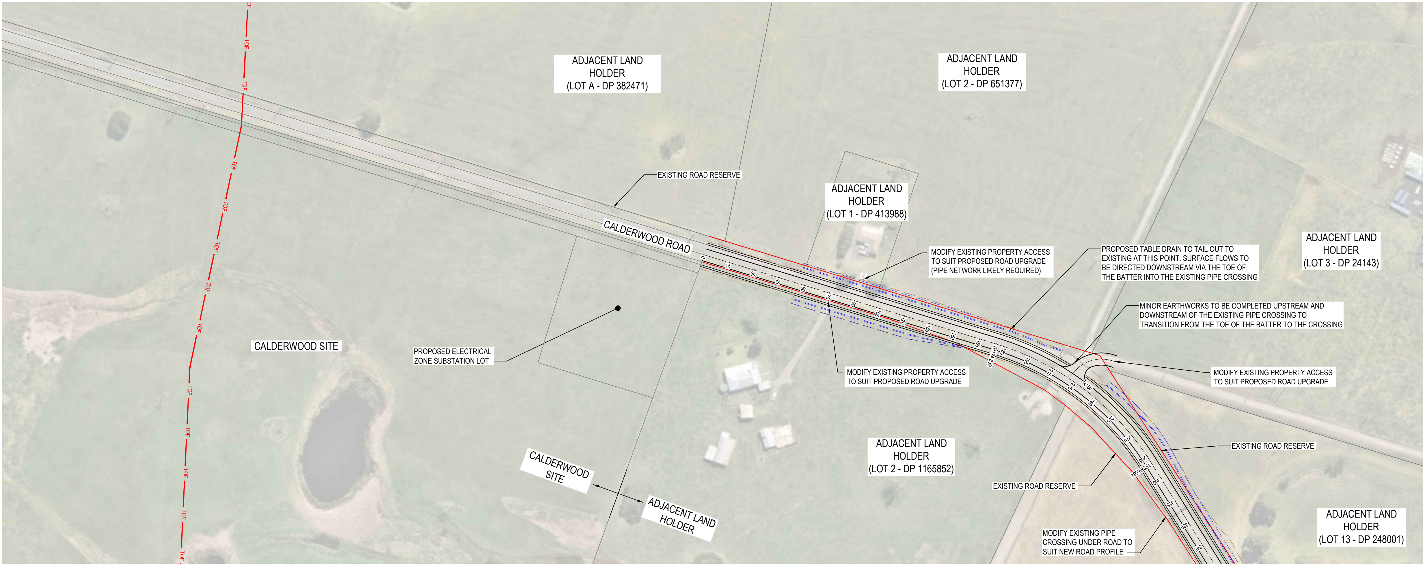
CALDERWOOD ROAD CONCEPT LAYOUT SCALE 1:1250
