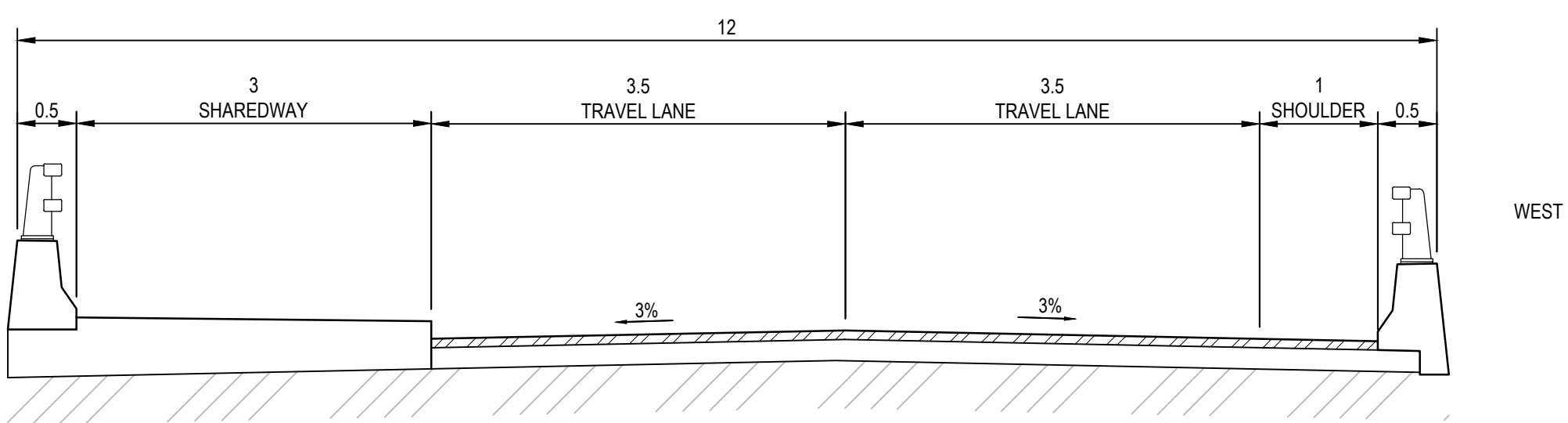
SECTION SCALE 1:50
