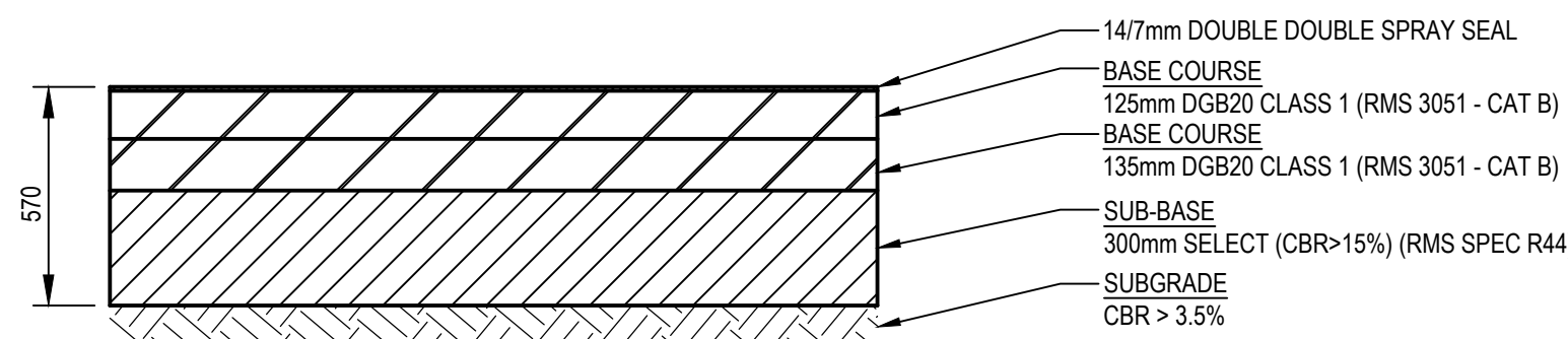
TYPICAL PAVEMENT DETAIL SCALE 1:20
