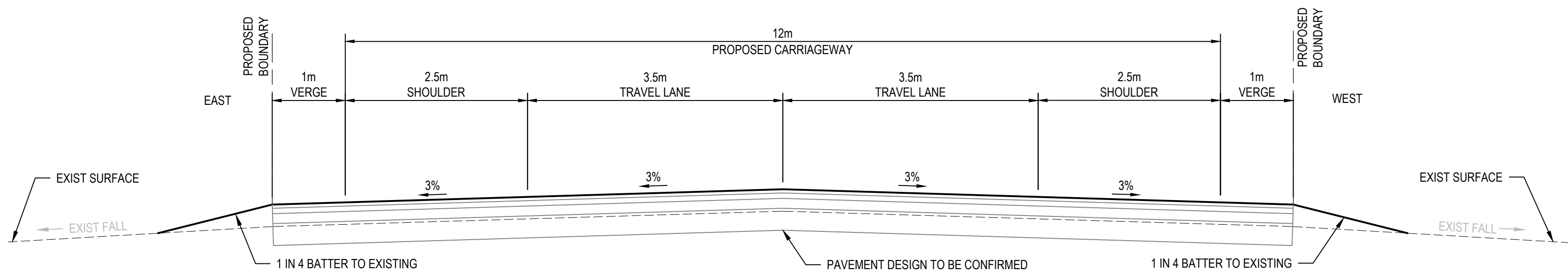
TYPICAL SECTION - TABLE DRAINS NOT REQUIRED SCALE 1:50
