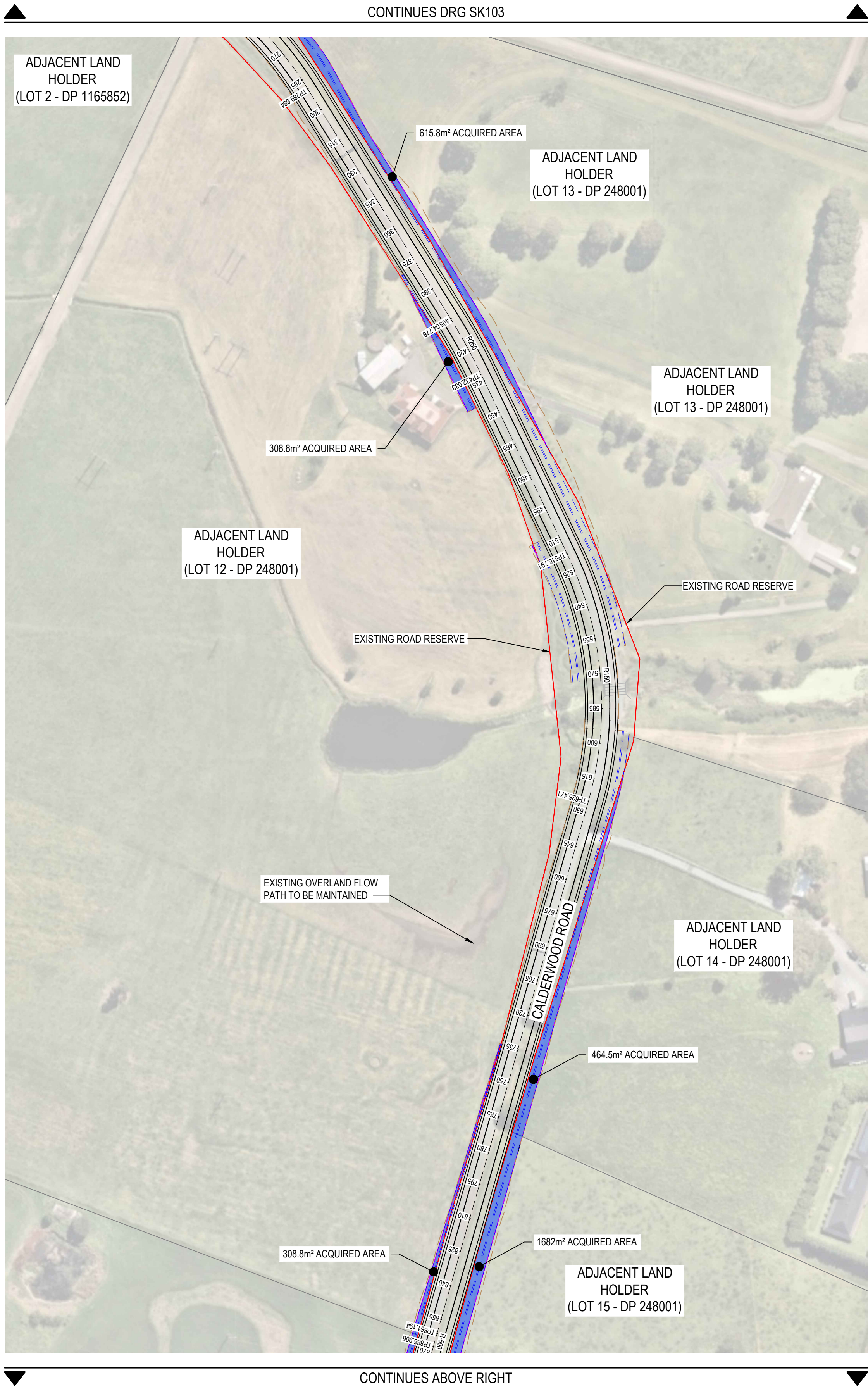
LAND ACQUISITION - CONCEPT LAYOUT SCALE 1:1250
