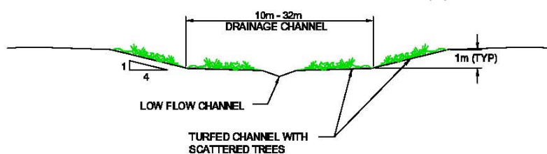
INDICATIVE DRAINAGE CROSS SECTION SCALE 1:200
