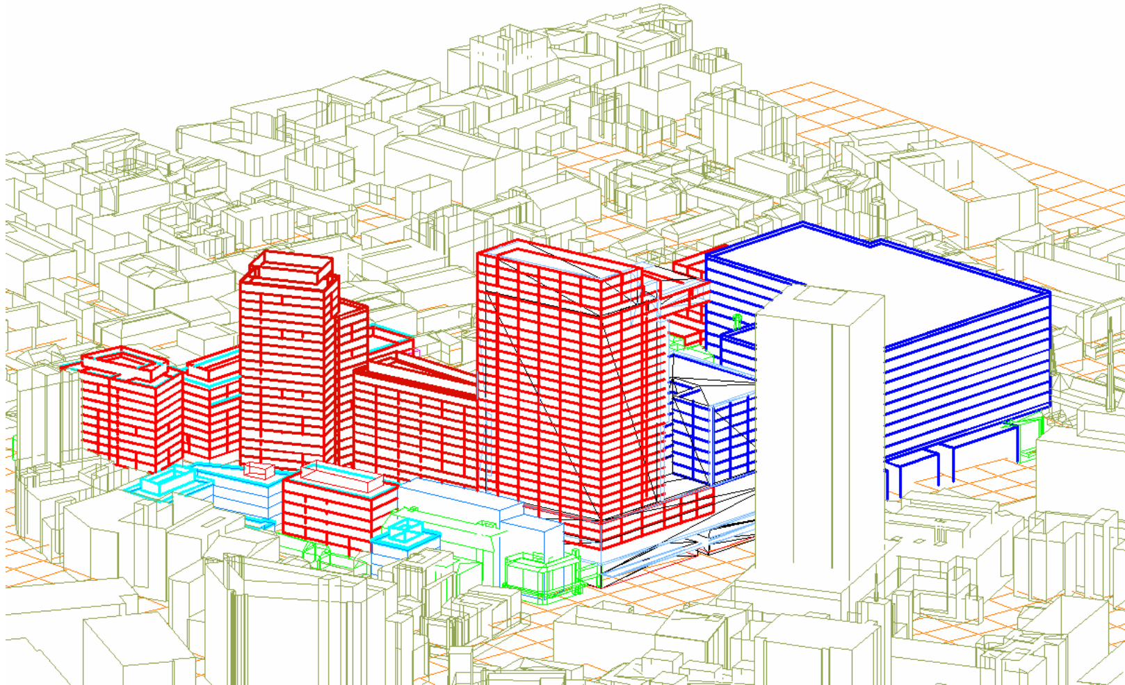
Figure 11 Development Sun's Eye View at 9.00 am on 21 June
