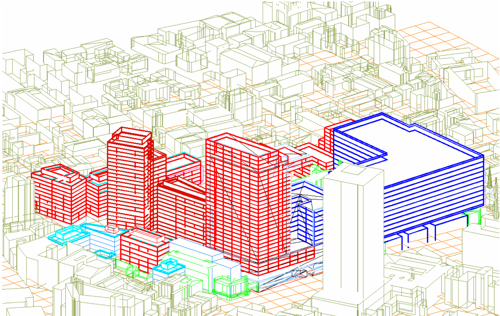
Figure 13 Development Sun's Eye View at 9.30 am on 21 June
