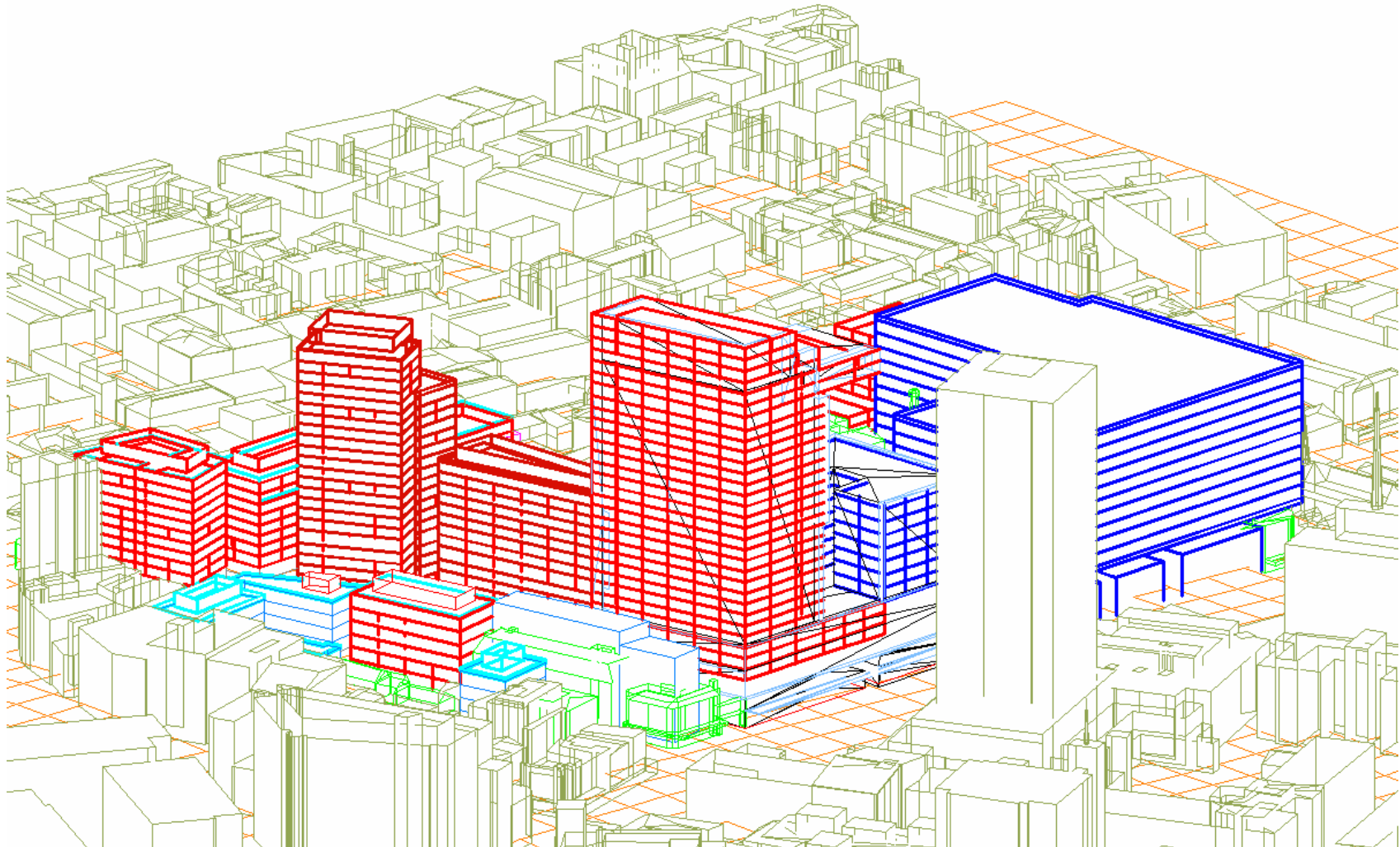
Figure 12 Development Sun's Eye View at 9.15 am on 21 June
