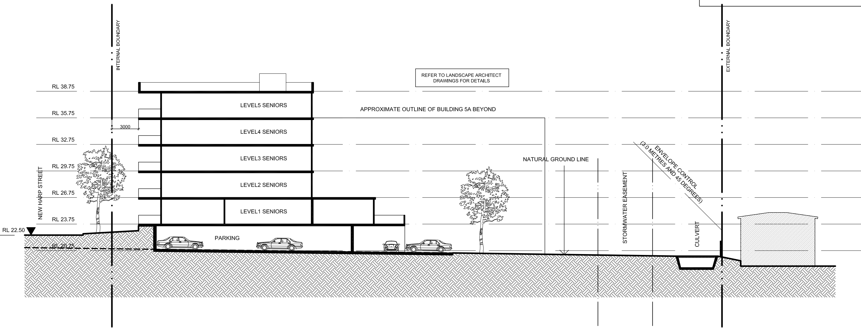
SECTION DD LOT 5B SENIORS LIVING COMPLEX
