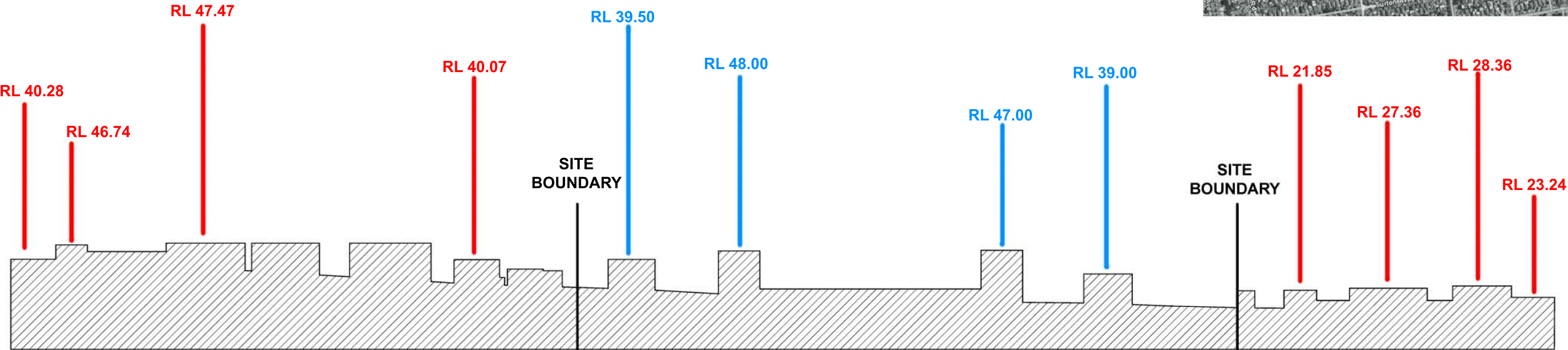
LONG SECTION
