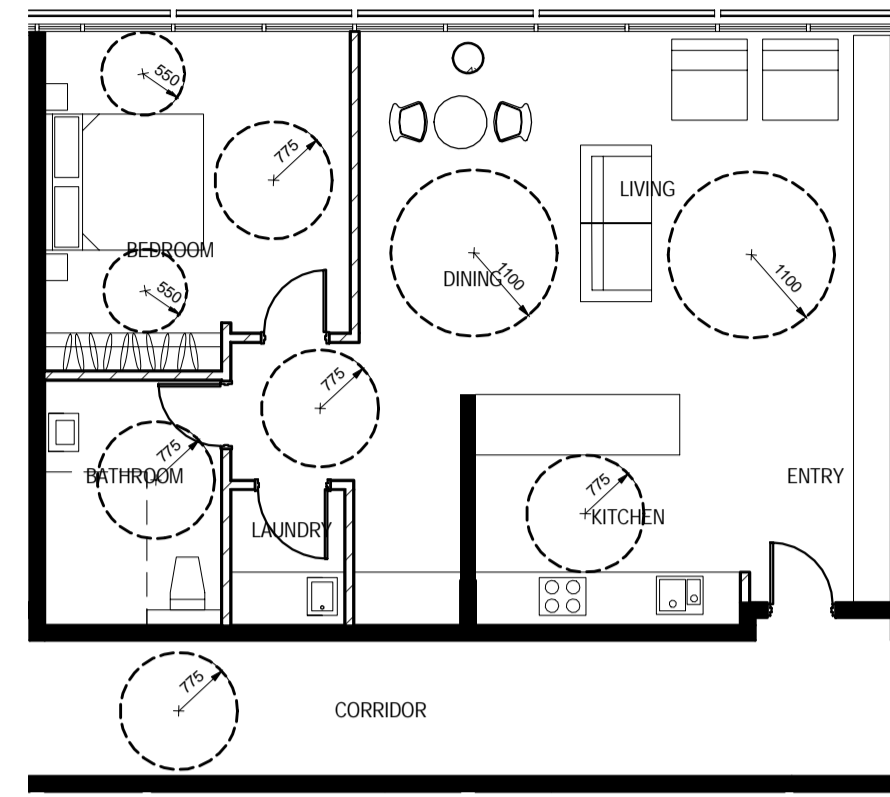
2 1 BEDROOM TYPE (Adaptable) Scale: 1 : 100
