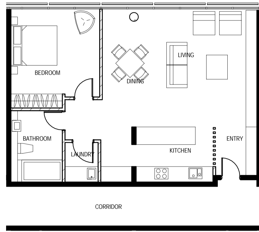
1 1 BEDROOM TYPE (Prior-Adaptable Conversion) Scale: 1 : 100
