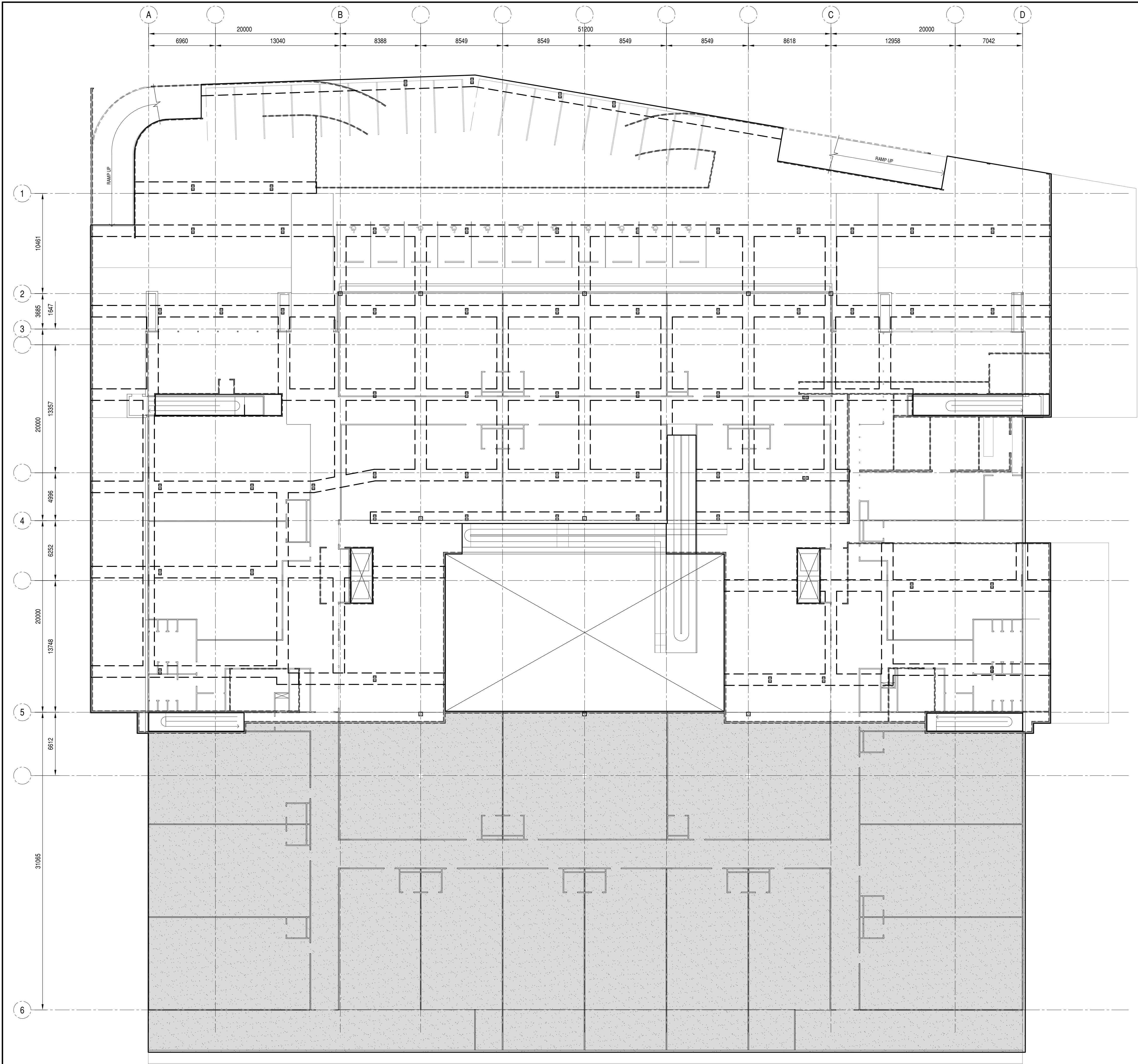
LEVEL 1 SLAB PLAN
