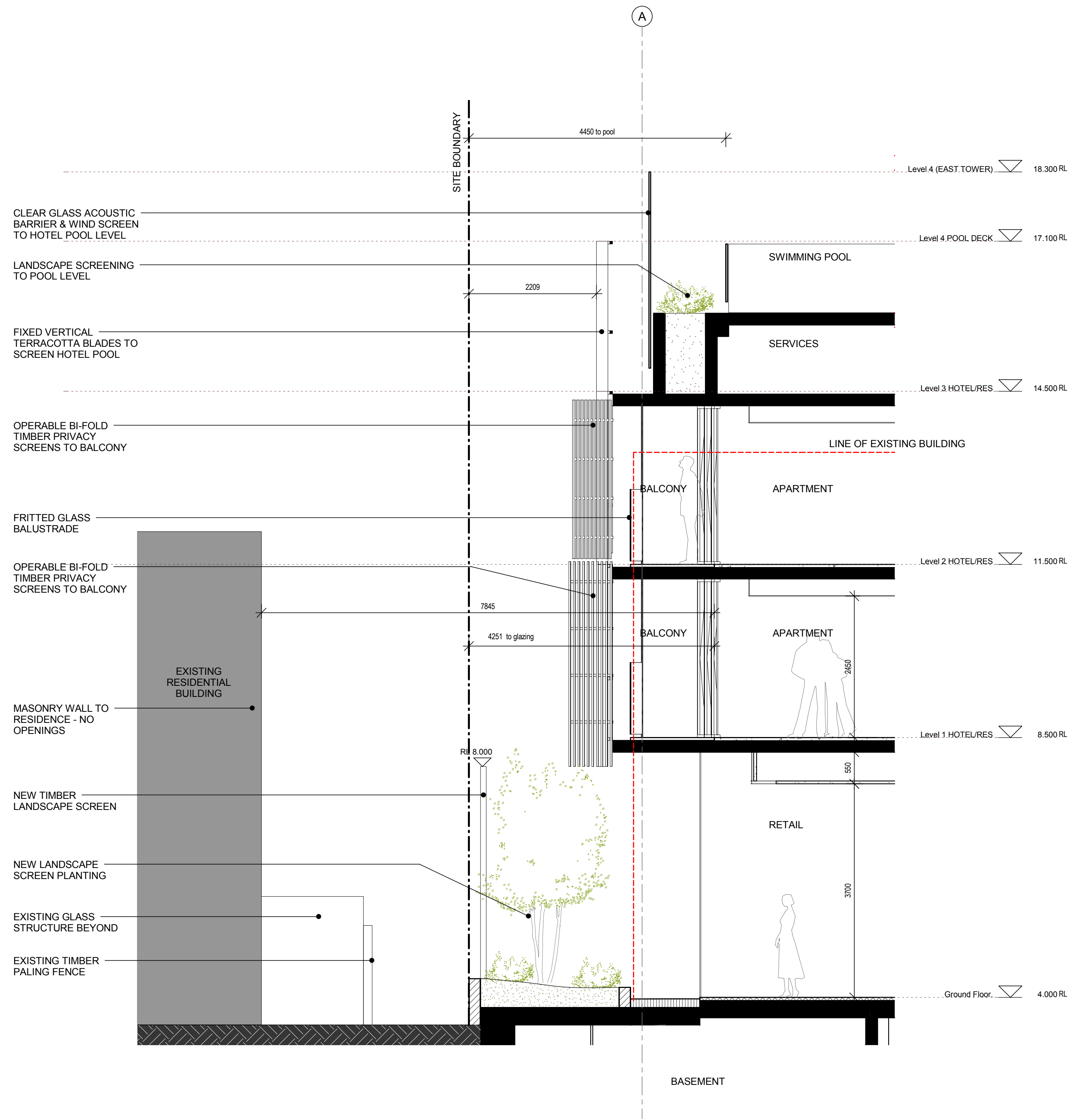
1 DETAIL SECTION 2-2 Scale: 1:50
