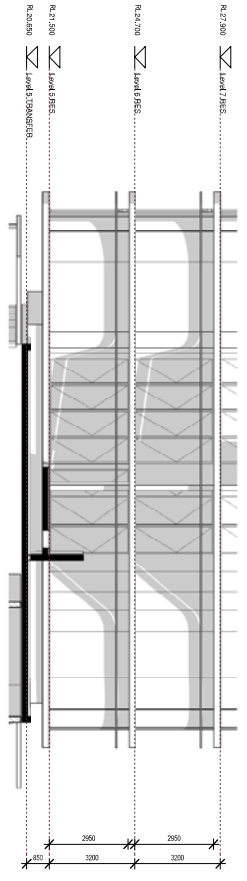
C WEST TOWER GLAZING - ELEV C Scale: 1 : 100
