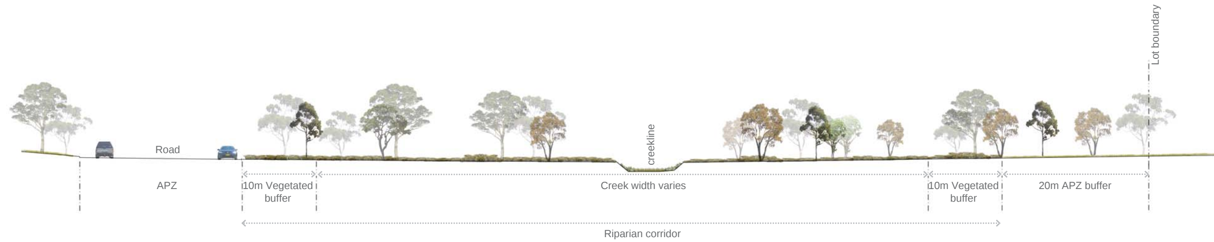
BLACK HILL RIPARIAN CORRIDOR TYPICAL SECTION A
