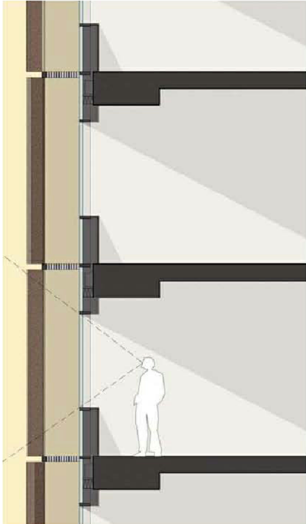
East / West Facade
