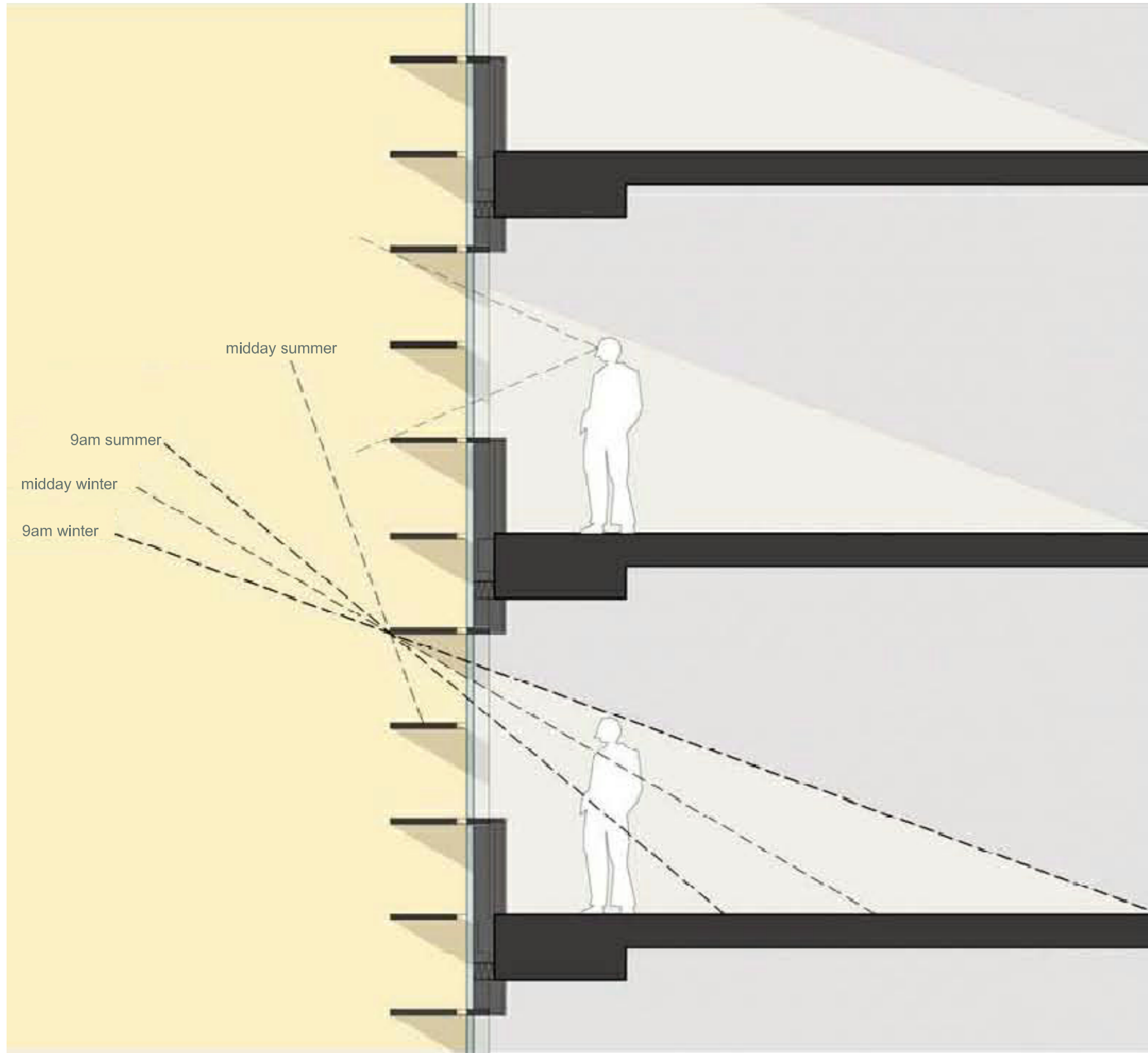
North Facade
