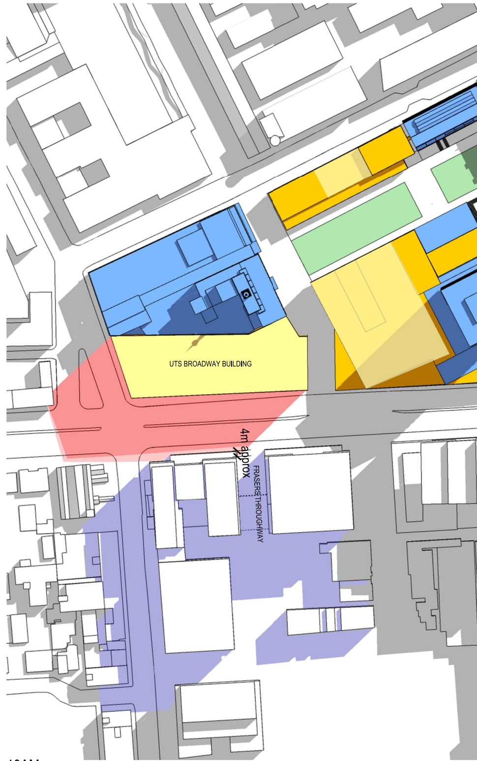
10AM EQUINOX (20 MARCH)
