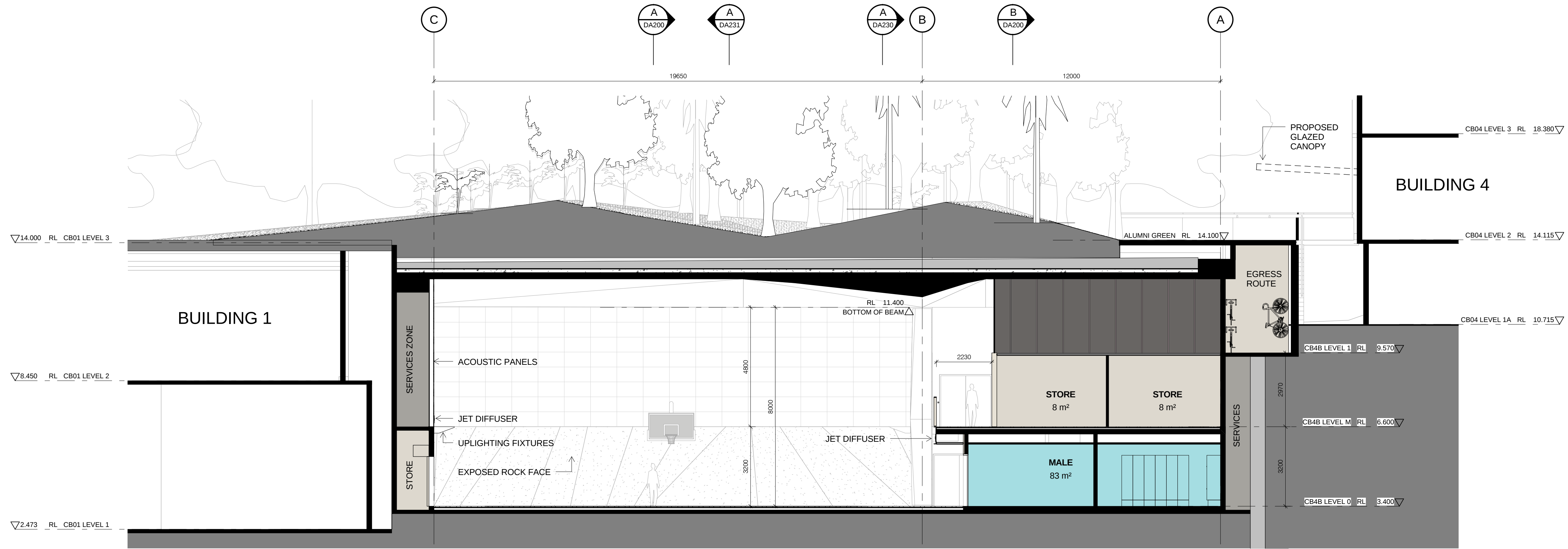
A SECTION NORTH-SOUTH 2 1 : 100
