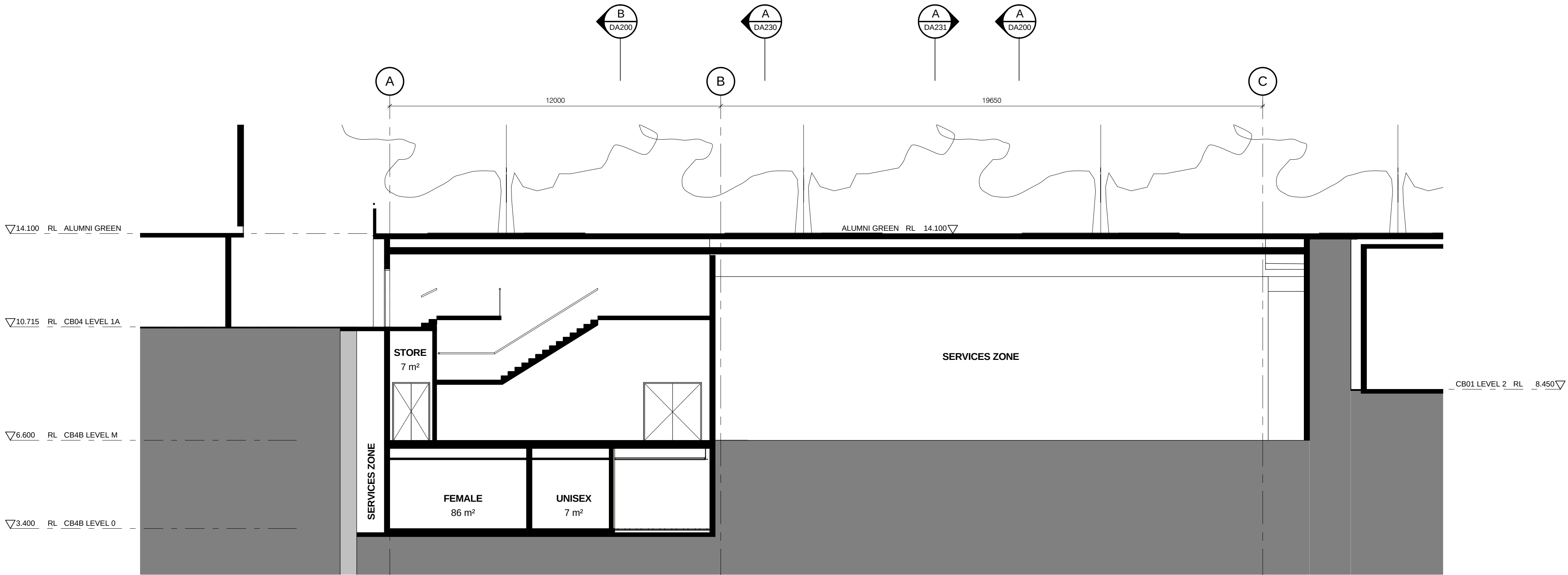
A NORTH-SOUTH SECTION (SERVICES) 1 : 100
