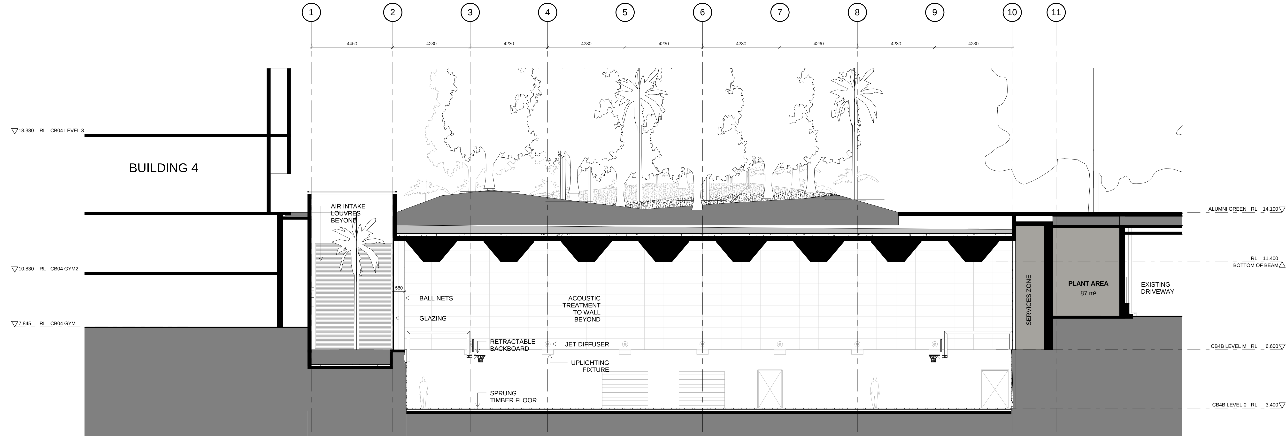
A ELEVATION SOUTH 1 : 100
