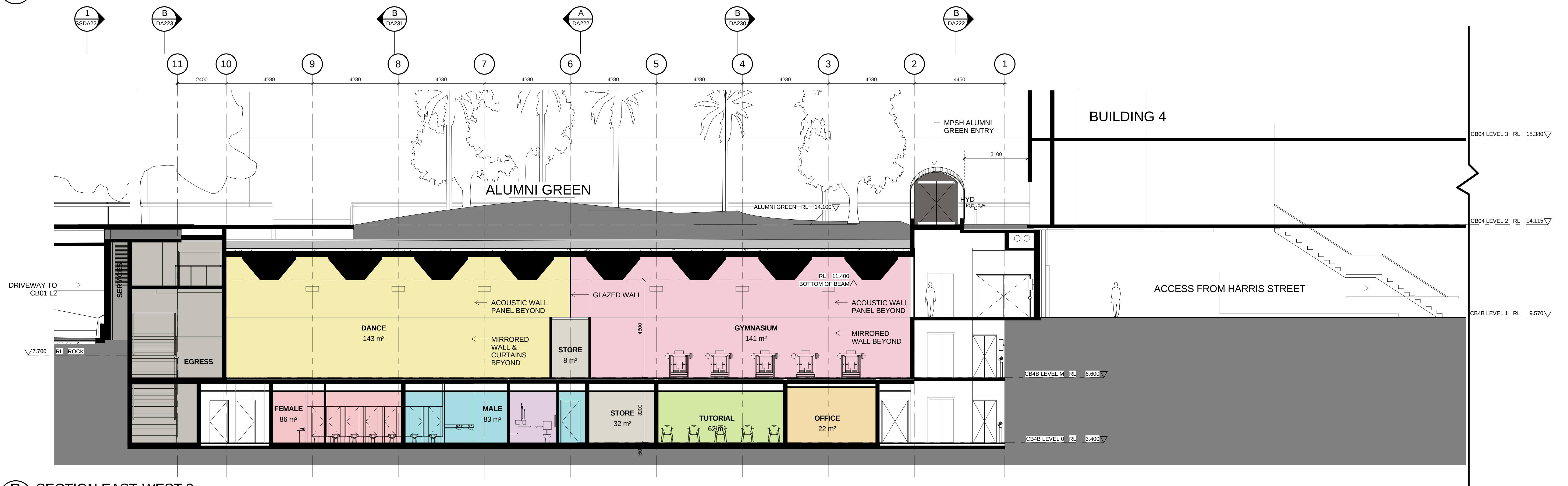
B SECTION EAST-WEST 2 1 : 100
