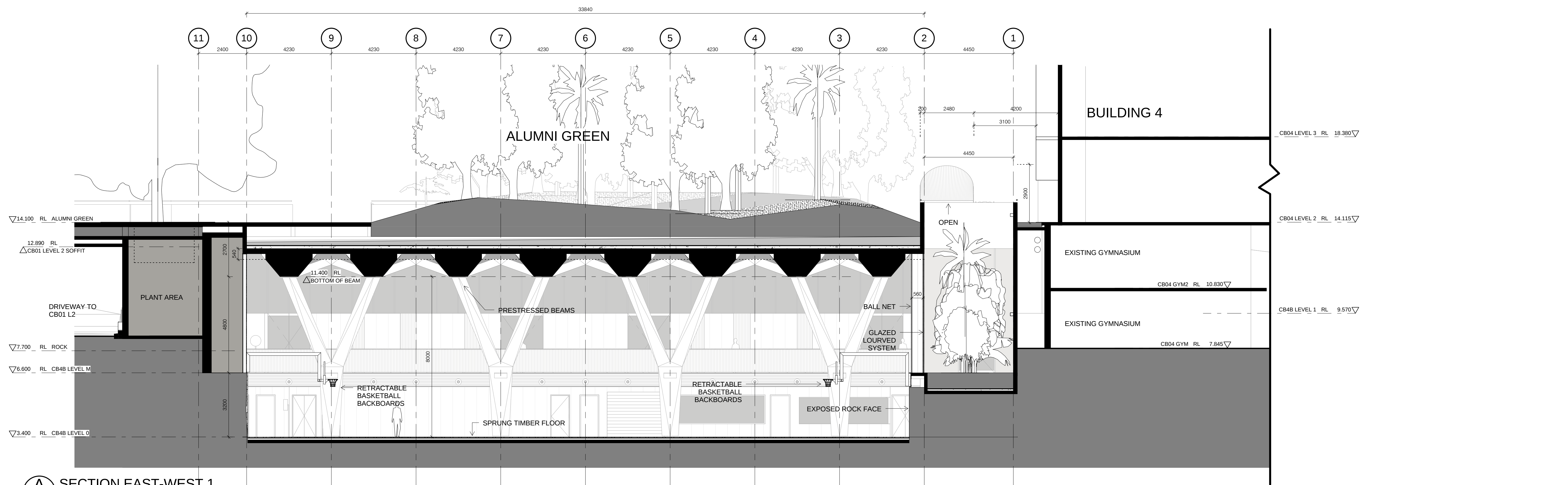
A SECTION EAST-WEST 1 1 : 100
