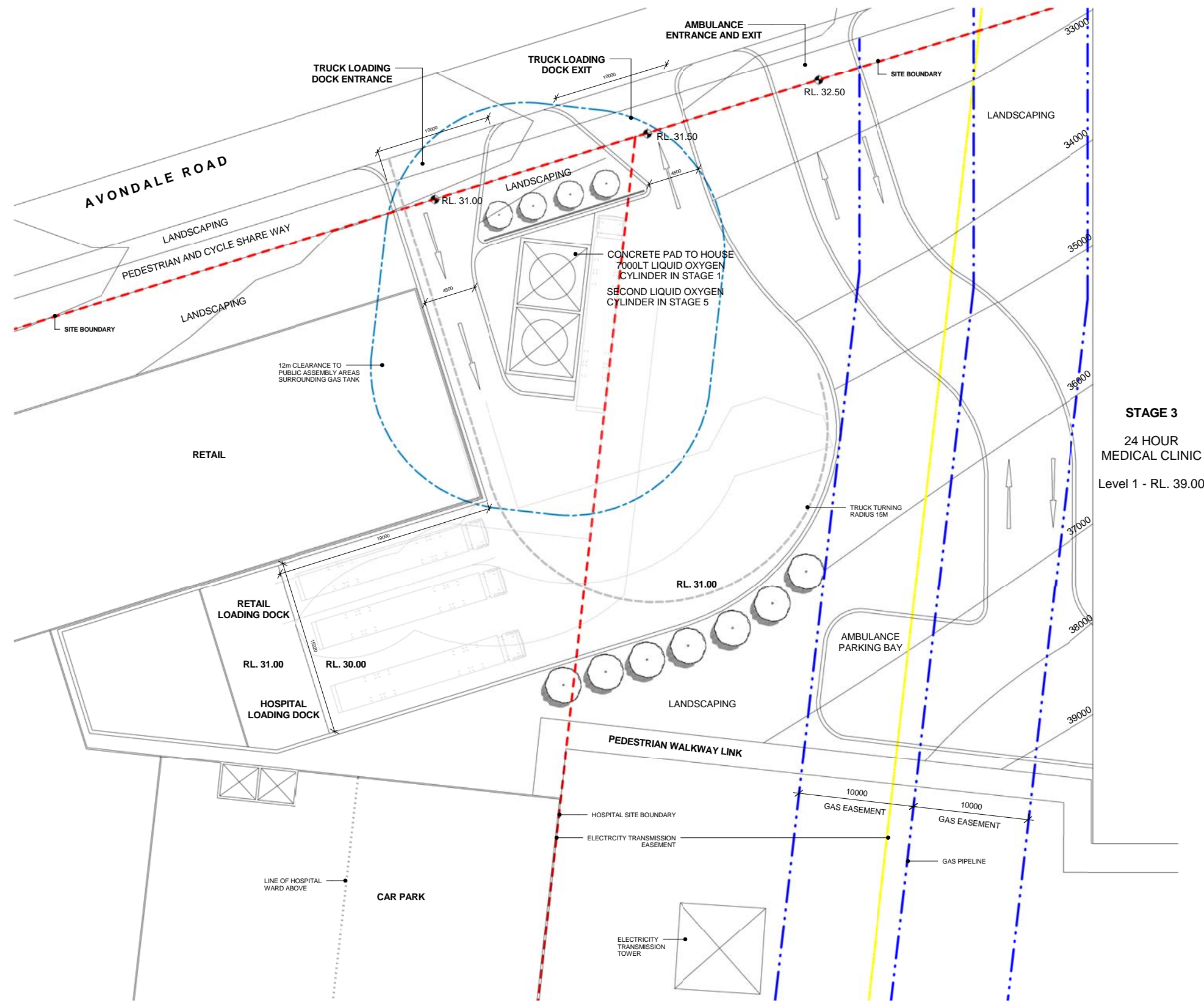
1 Liquid Oxygen Cylinder and Loading Dock 1:200
