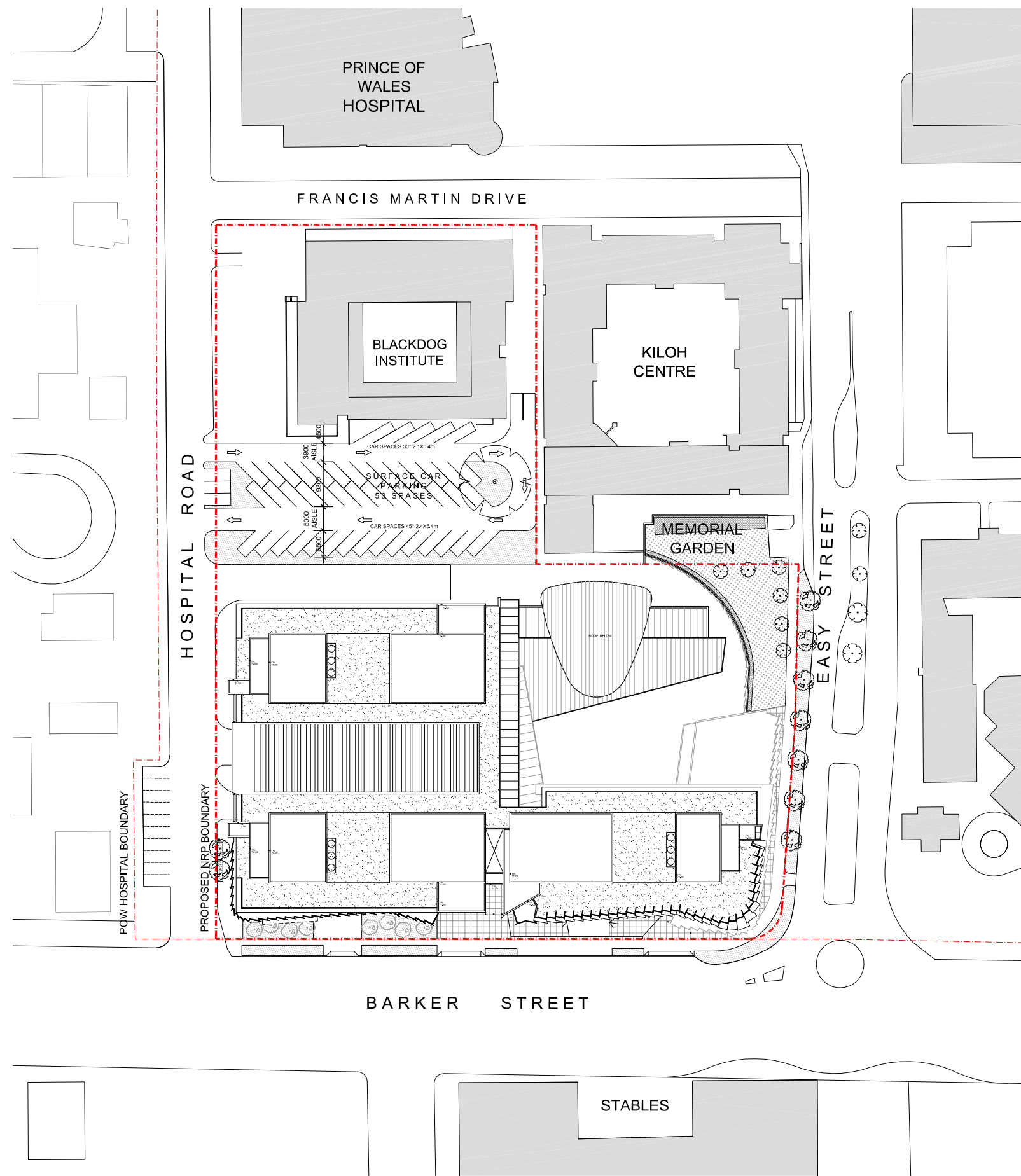
01 PROPOSED SITE PLAN 1:500
