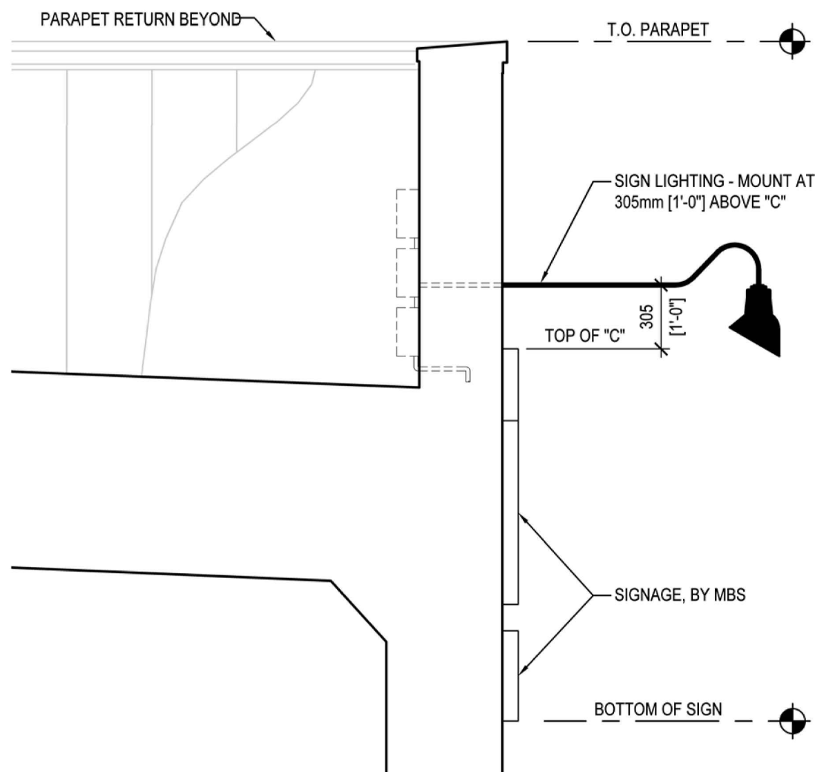
TYPE BUILDING SIGNAGE AND LIGHT SECTION SCALE: 1:25
