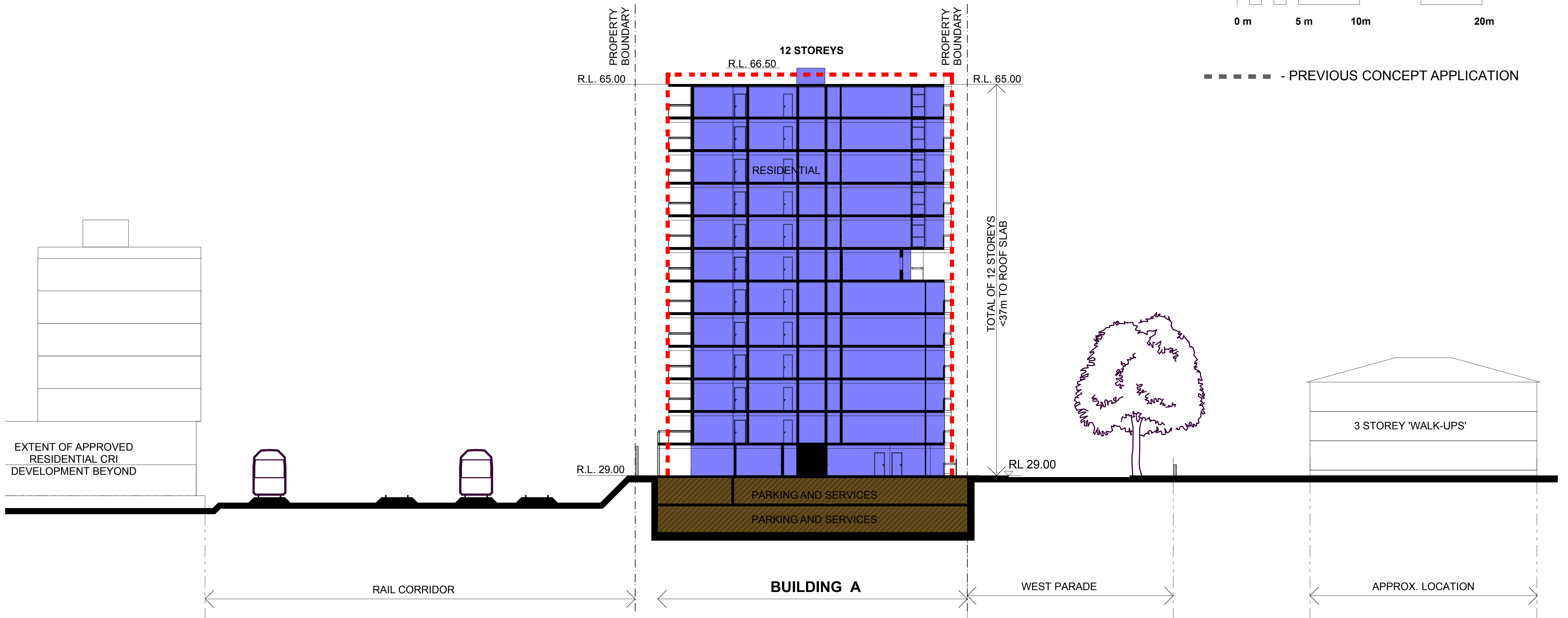
SECTION B-B ( EAST - WEST )
