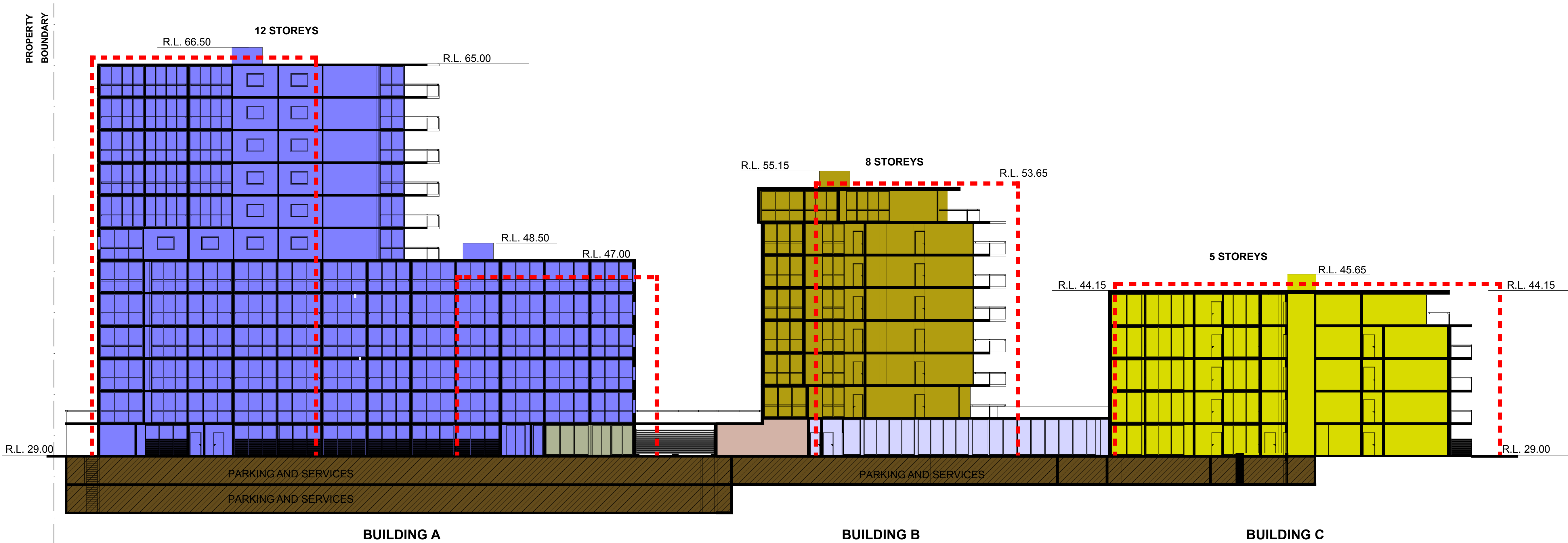
SECTION A-A ( NORTH - SOUTH )
