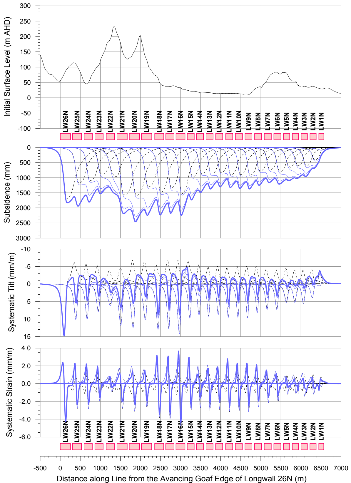
Figure 5.2 Predicted Subsidence, Systematic Tilt and Systematic Strain Profiles Prediction Line 1
