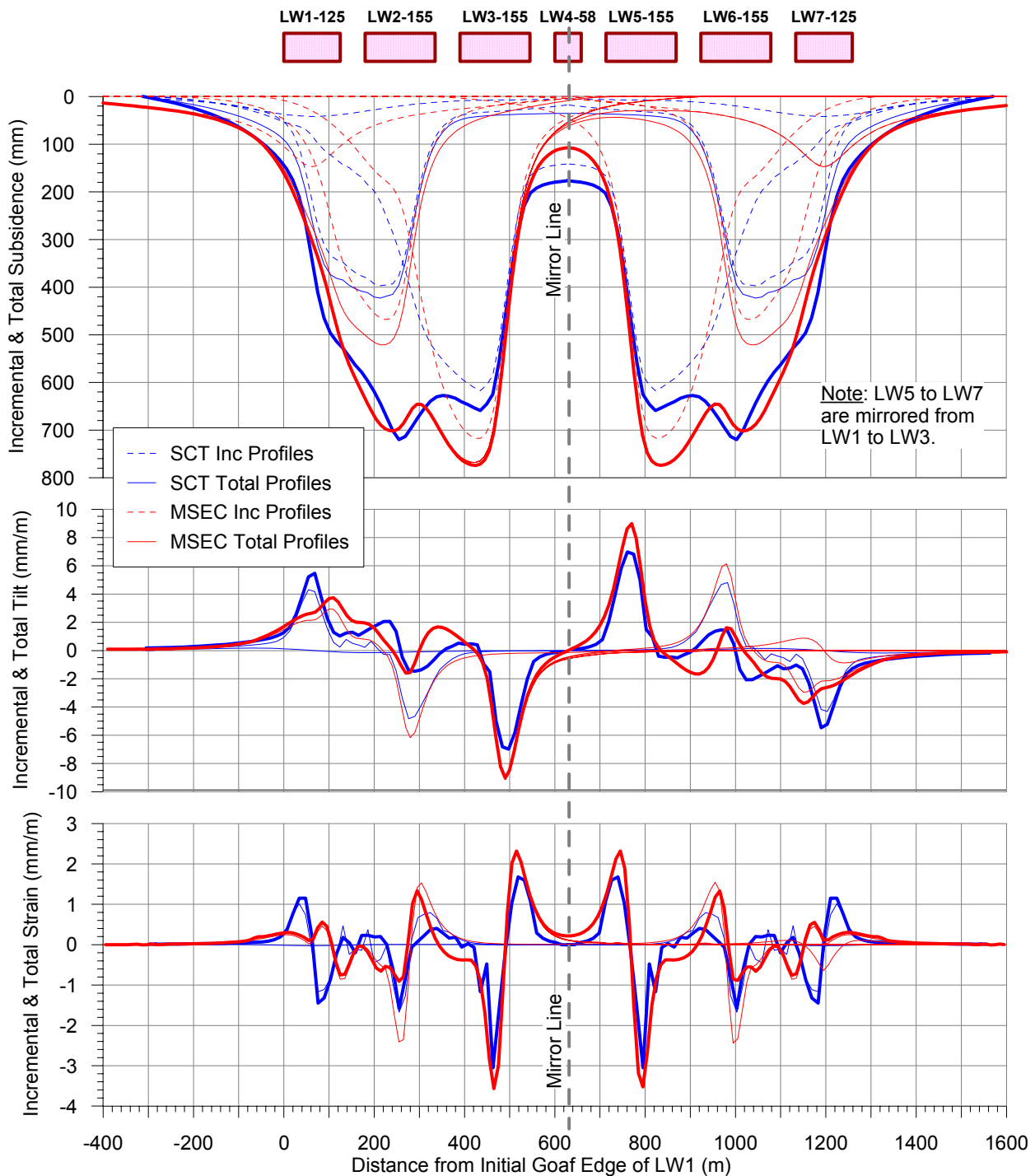
Figure 3.1 Comparison of Predicted Profiles for the Hue Hue Case
