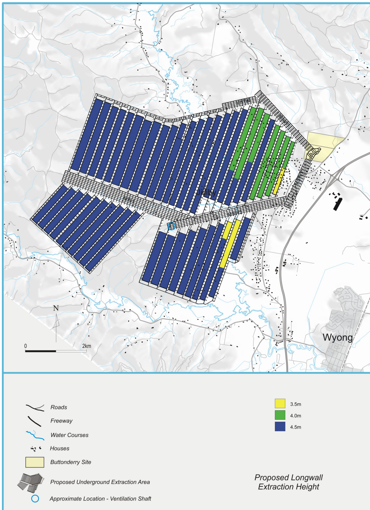
Figure 4.2 Current layout showing areas of various extraction heights
