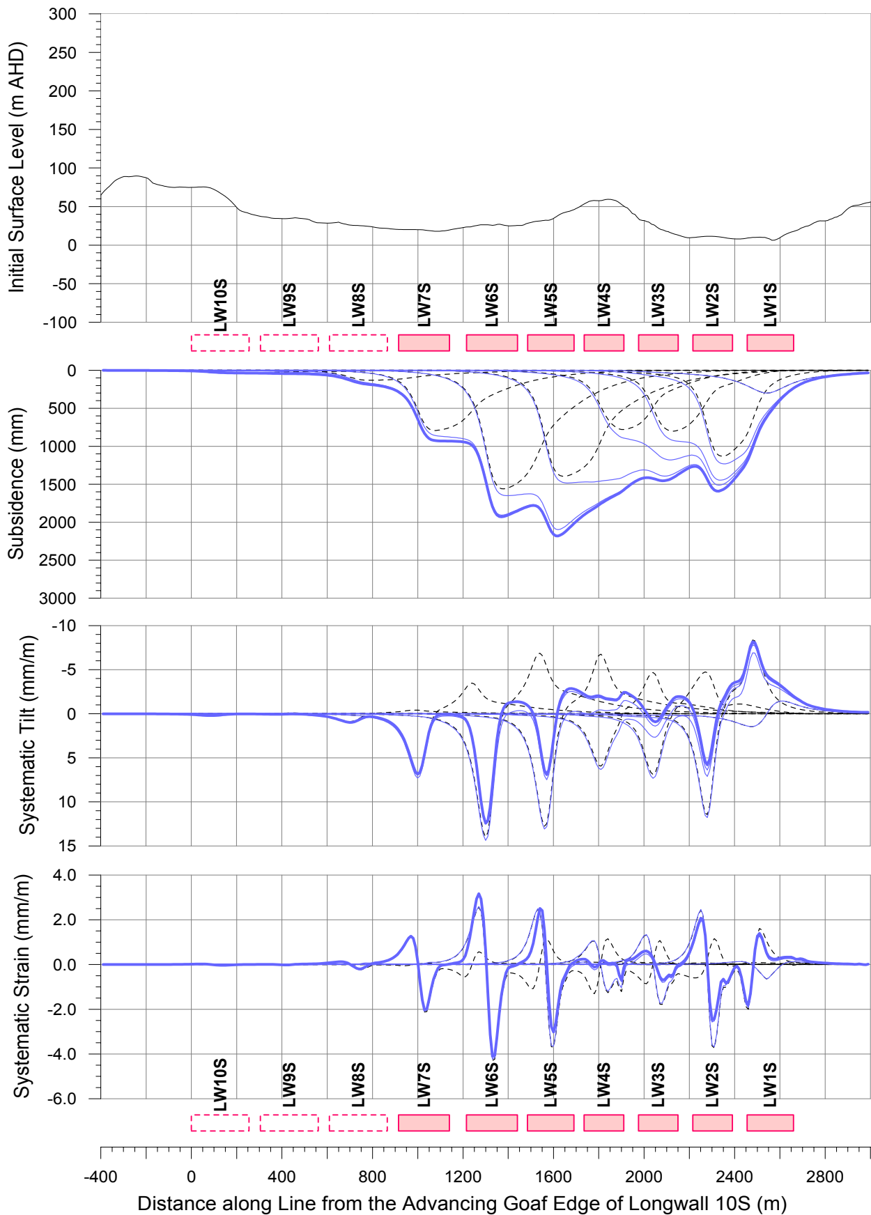
Figure 5.5 Predicted Subsidence, Systematic Tilt and Systematic Strain Profiles Prediction Line 4
