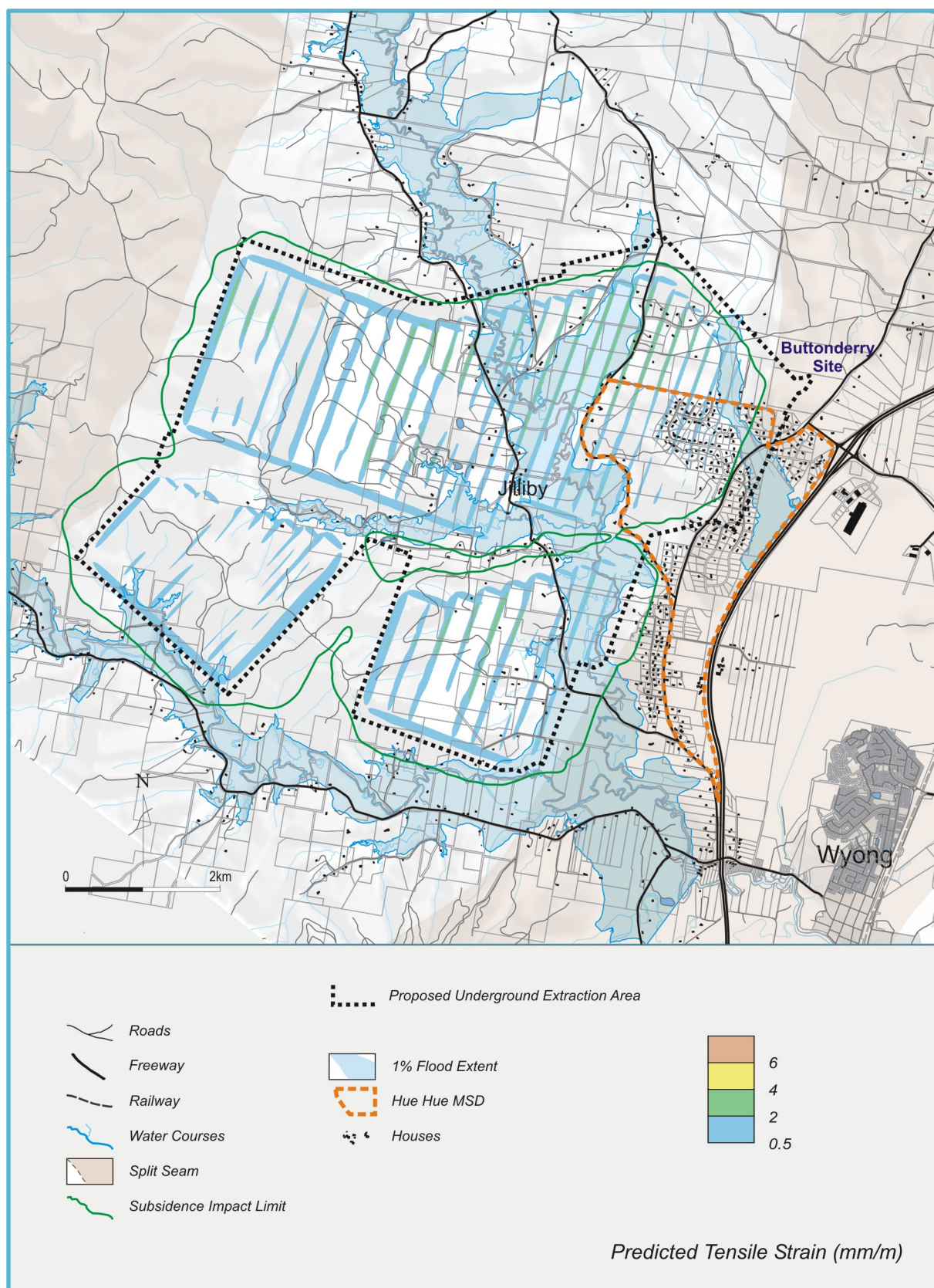
Figure 5.9 Predicted Total Tensile Strain
