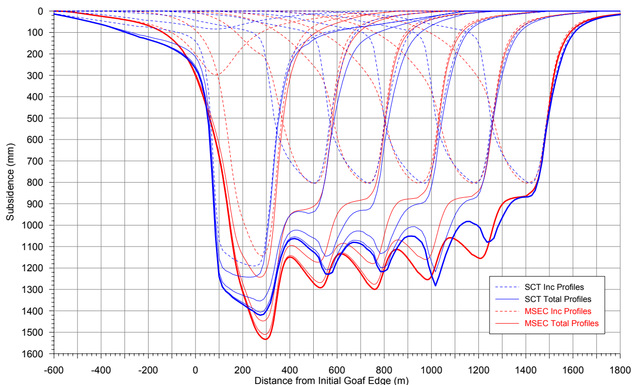
Figure 3.2 Comparison of Predicted Profiles for the Valley Case
