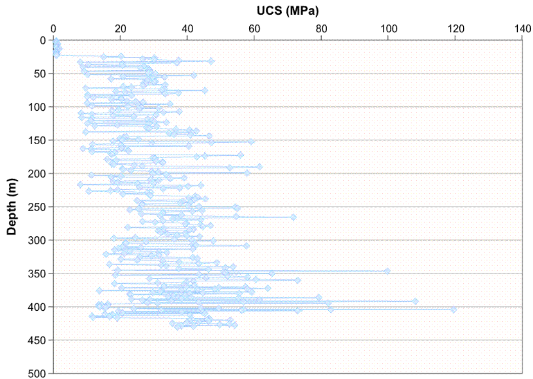
Figure 2.10 Typical Distribution in UCS of Overburden in W2CP Area
