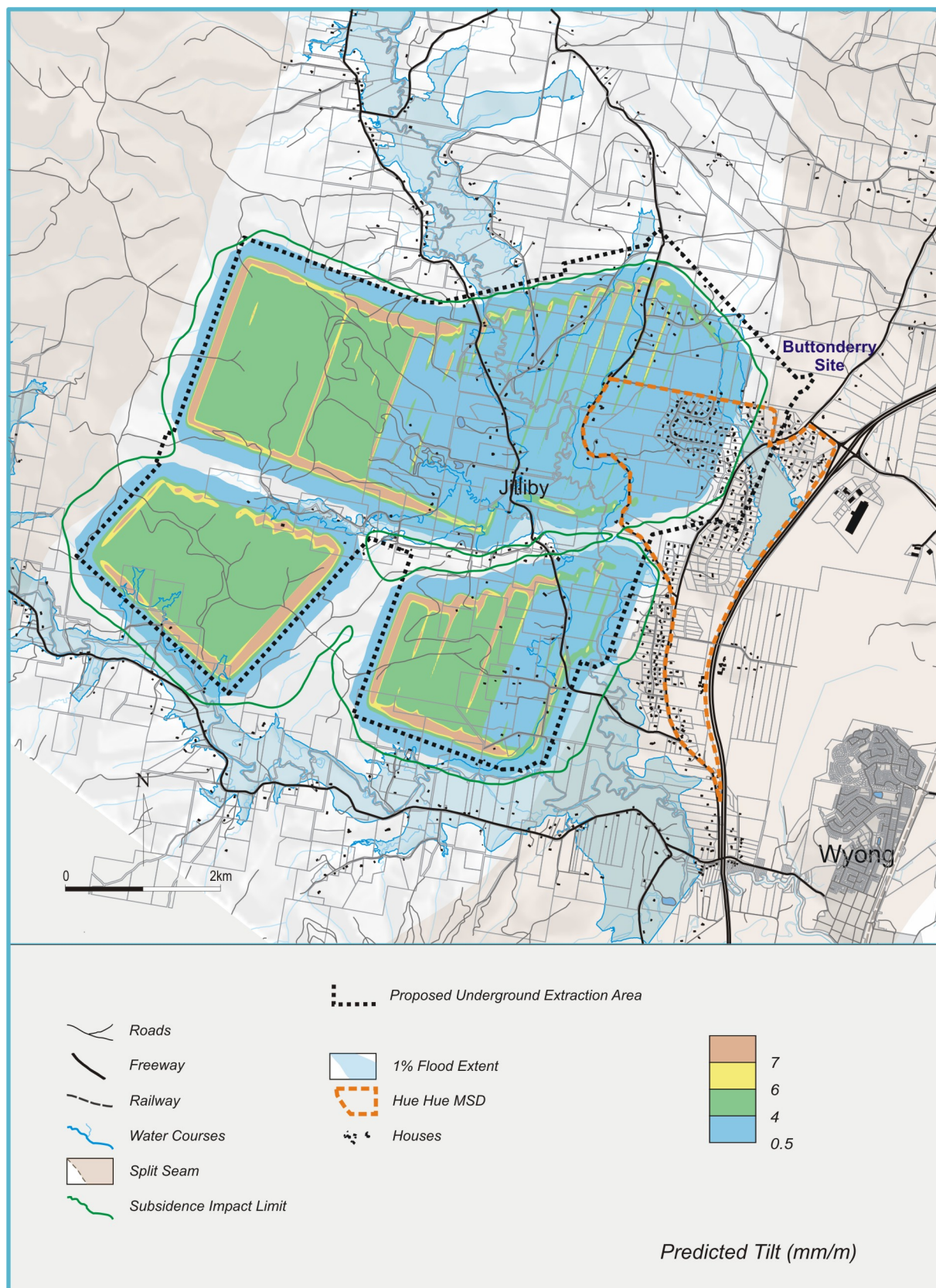
Figure 5.7 Predicted Total Tilt
