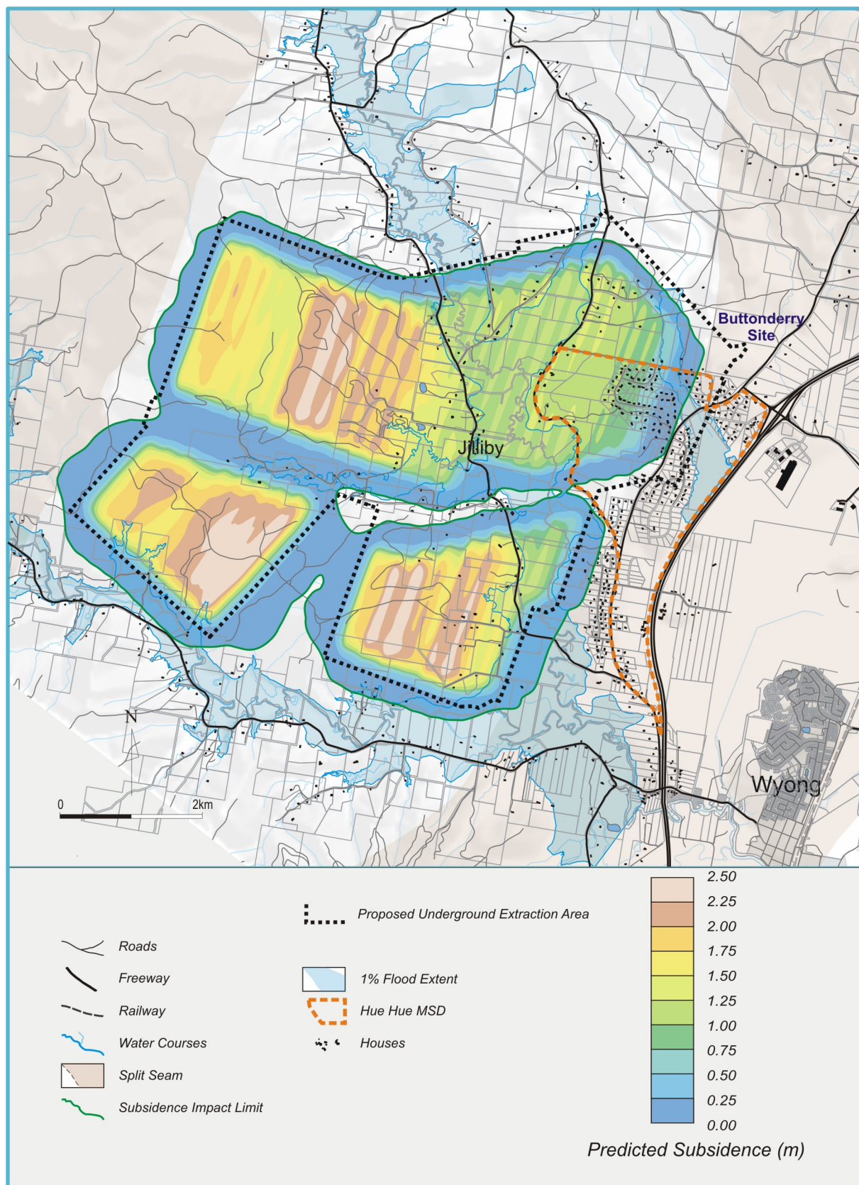
Figure 5.6 Predicted Total Subsidence
