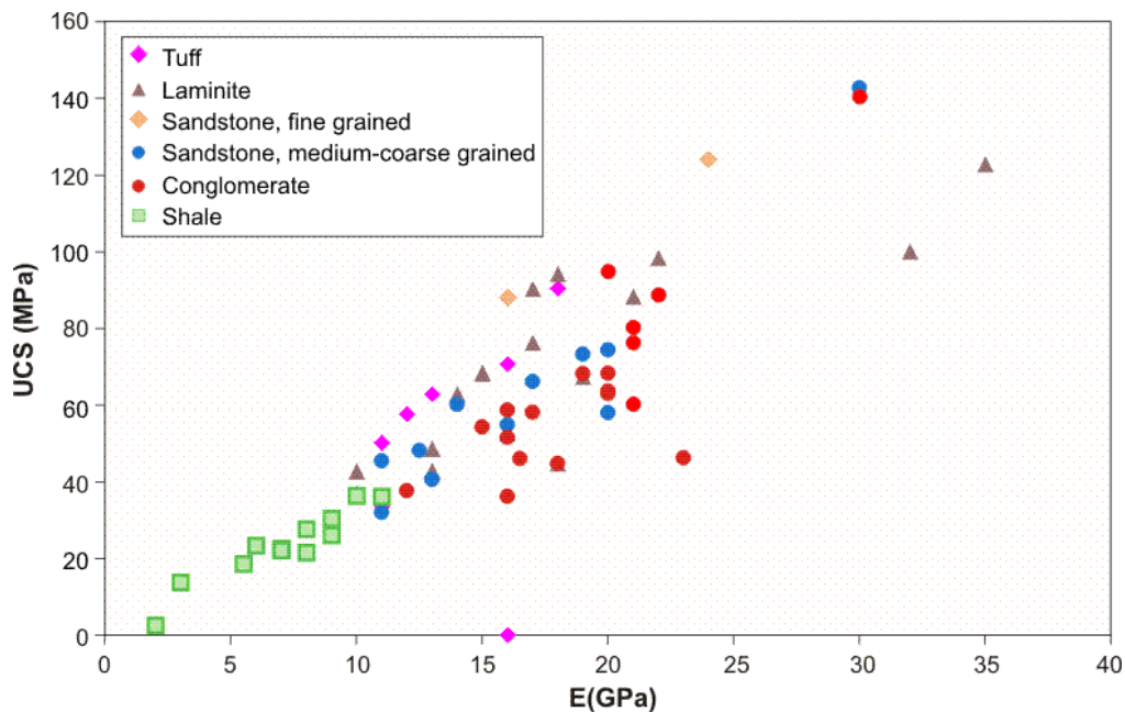
Figure 2.11 Typical Strength Characteristics of Rock Types in W2CP Area
