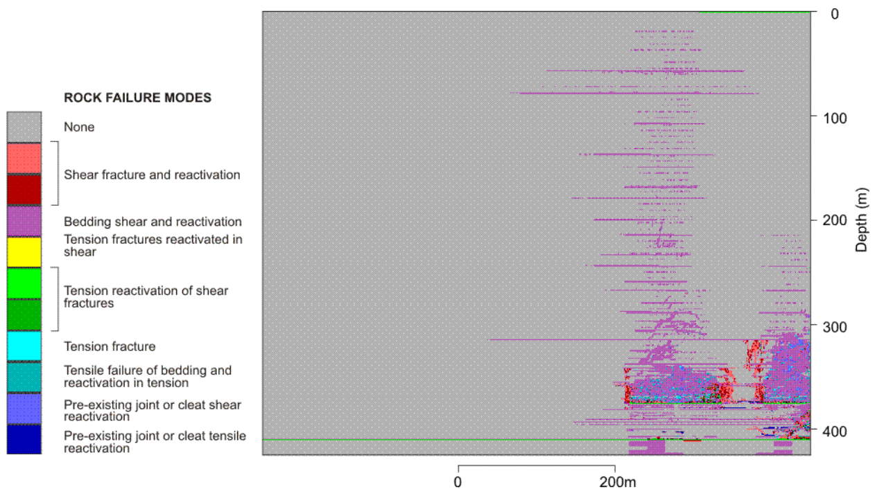
Figure 2.8 Modelled Rock Fracture Development after South Bulli Longwalls 1 and 2
