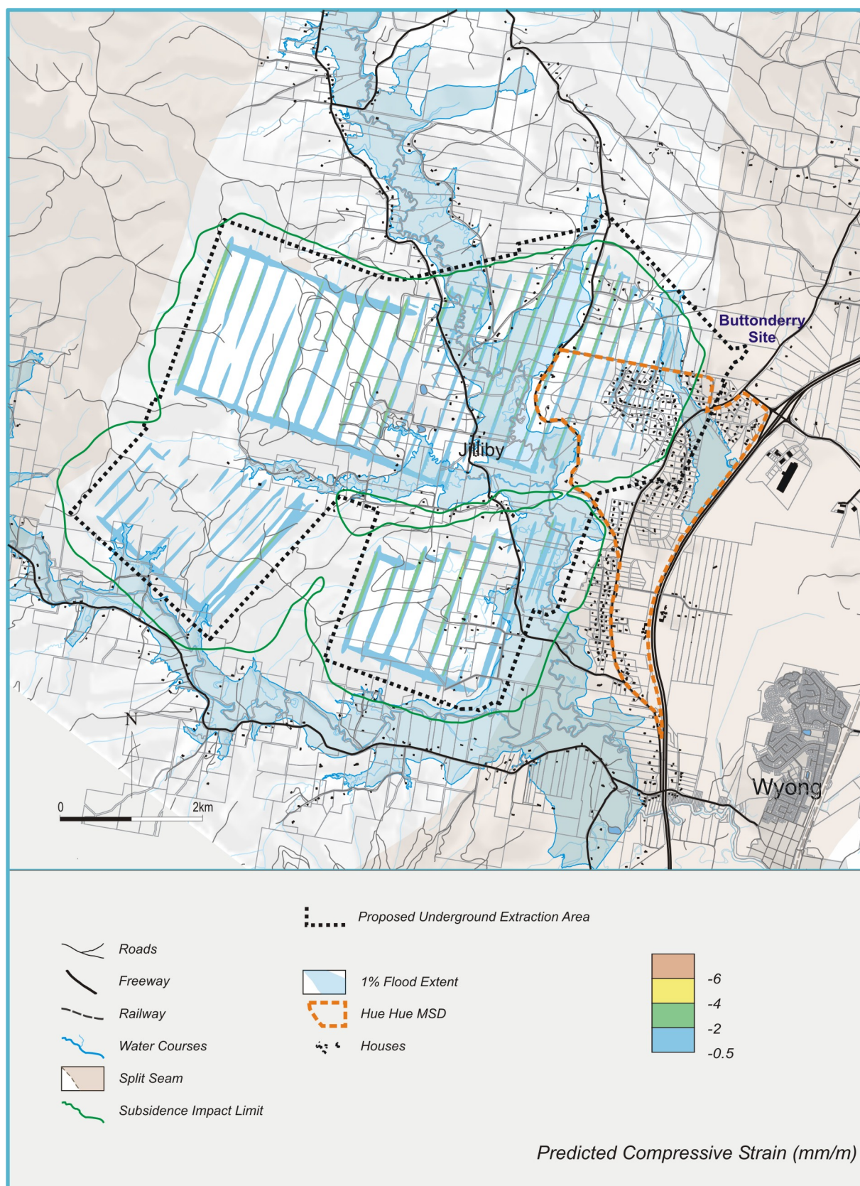
Figure 5.8 Predicted Total Compressive Strain
