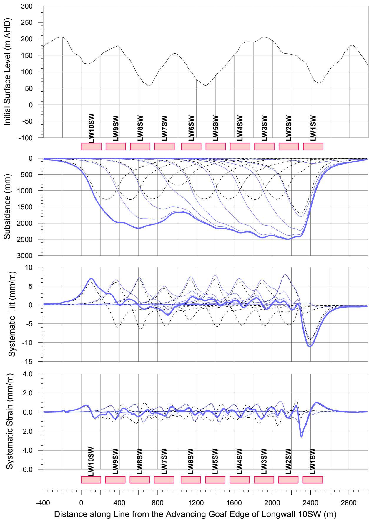
Figure 5.4 Predicted Subsidence, Systematic Tilt and Systematic Strain Profiles Prediction Line 3
