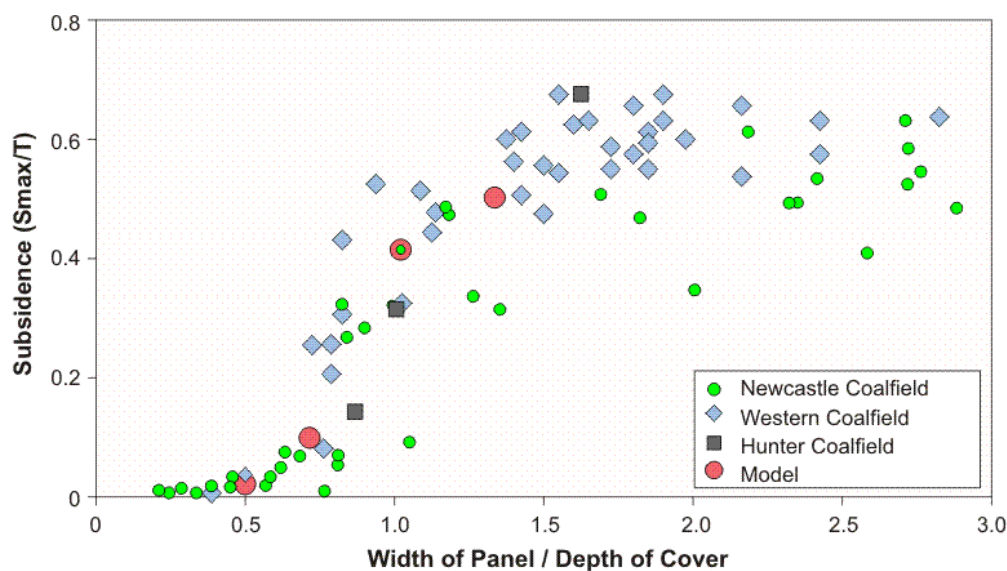
Figure 2.1 Regional Subsidence Data for Newcastle, Hunter and Western Coalfields
