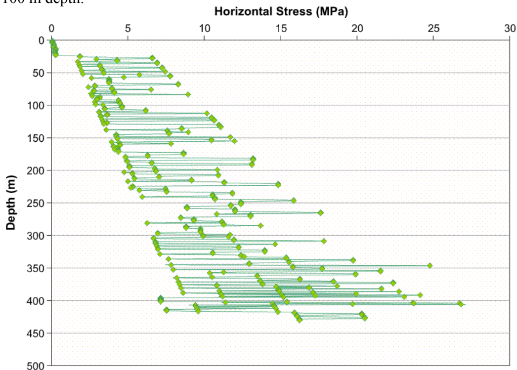
Figure 2.12 Modelled Horizontal Stress vs Depth in W2CP Area
