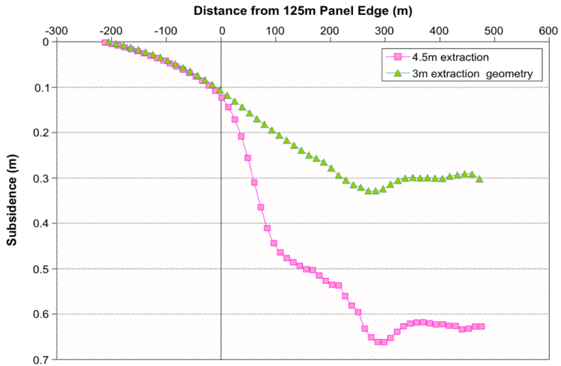
Figure 2.26 Modelled Subsidence Profiles for the Hue Hue 3.0 m and 4.5 m Cases
