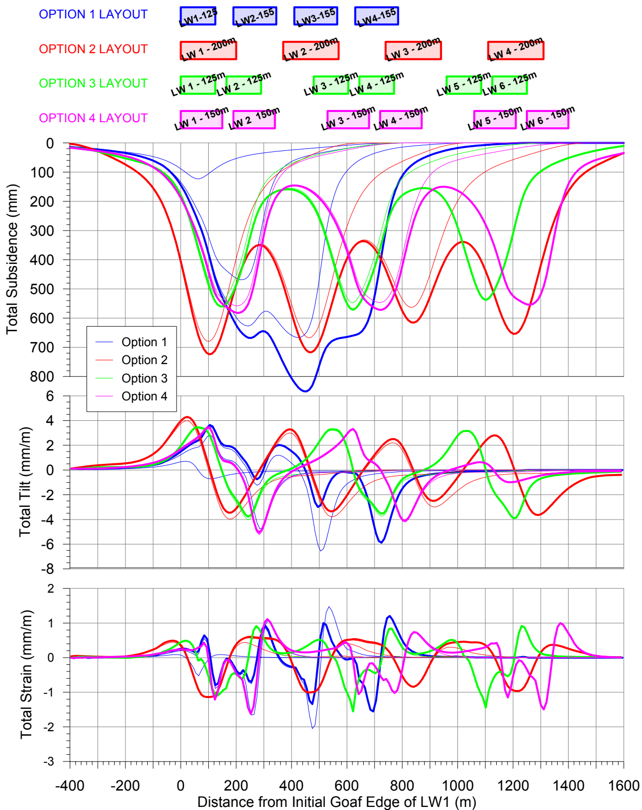
Figure 4.1 Comparison of Predicted Systematic Subsidence Profiles for Options 1 to 4
