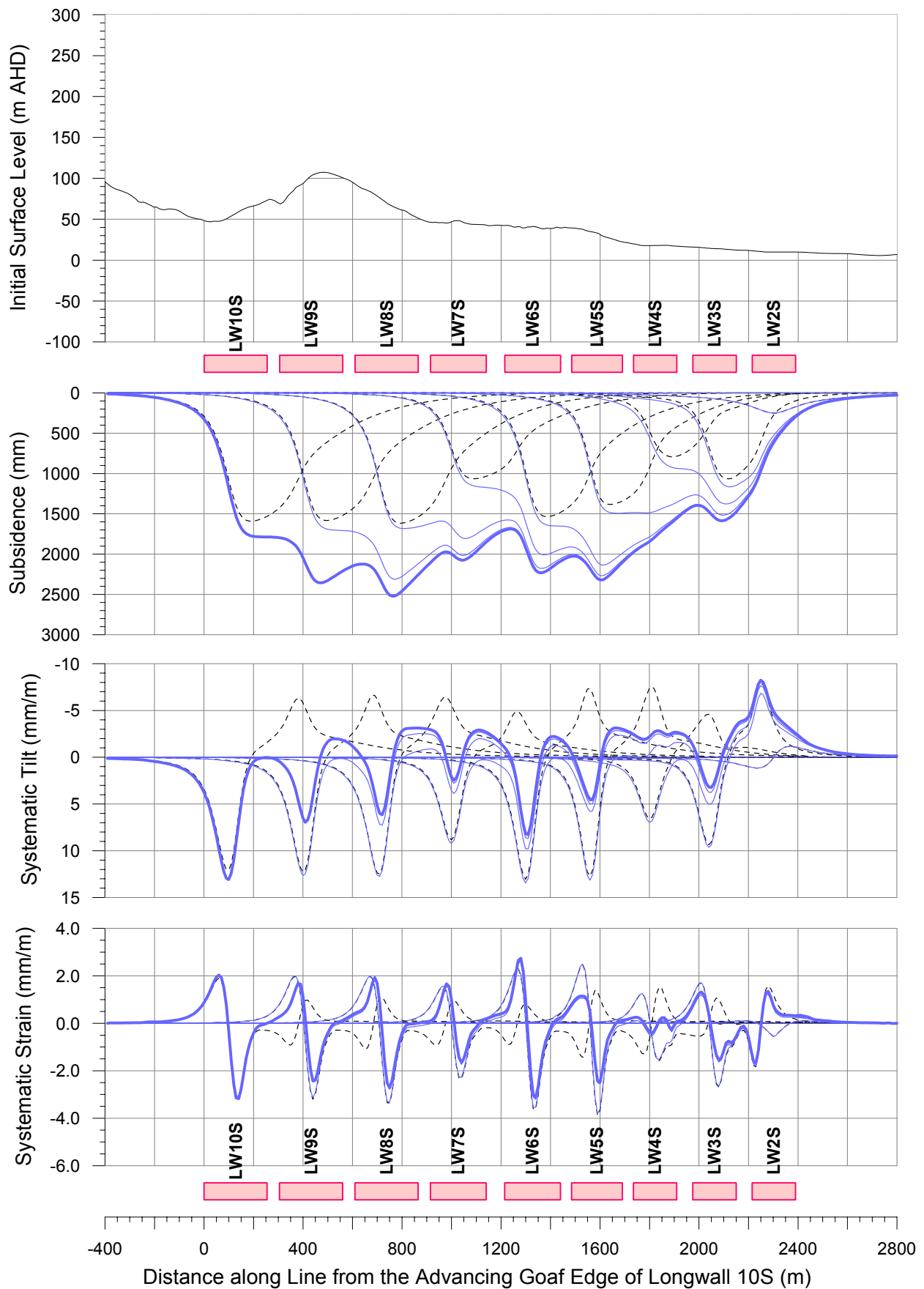
Figure 5.3 Predicted Subsidence, Systematic Tilt and Systematic Strain Profiles Prediction Line 2
