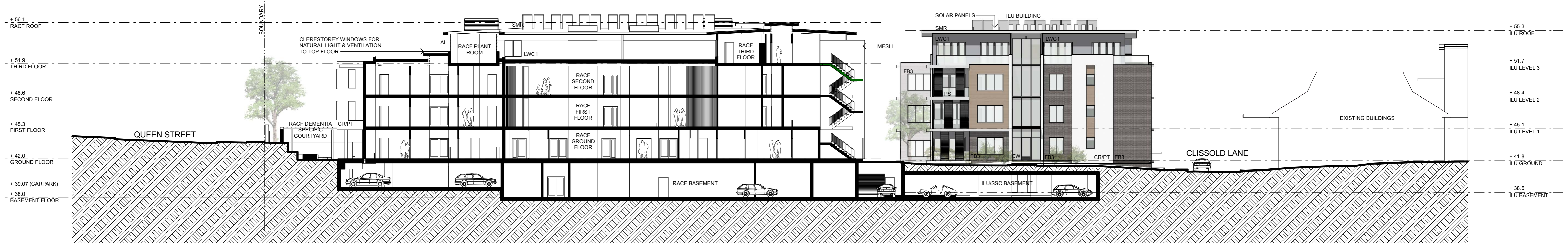
08 SECTION 08 SCALE 1:200 @ A1
