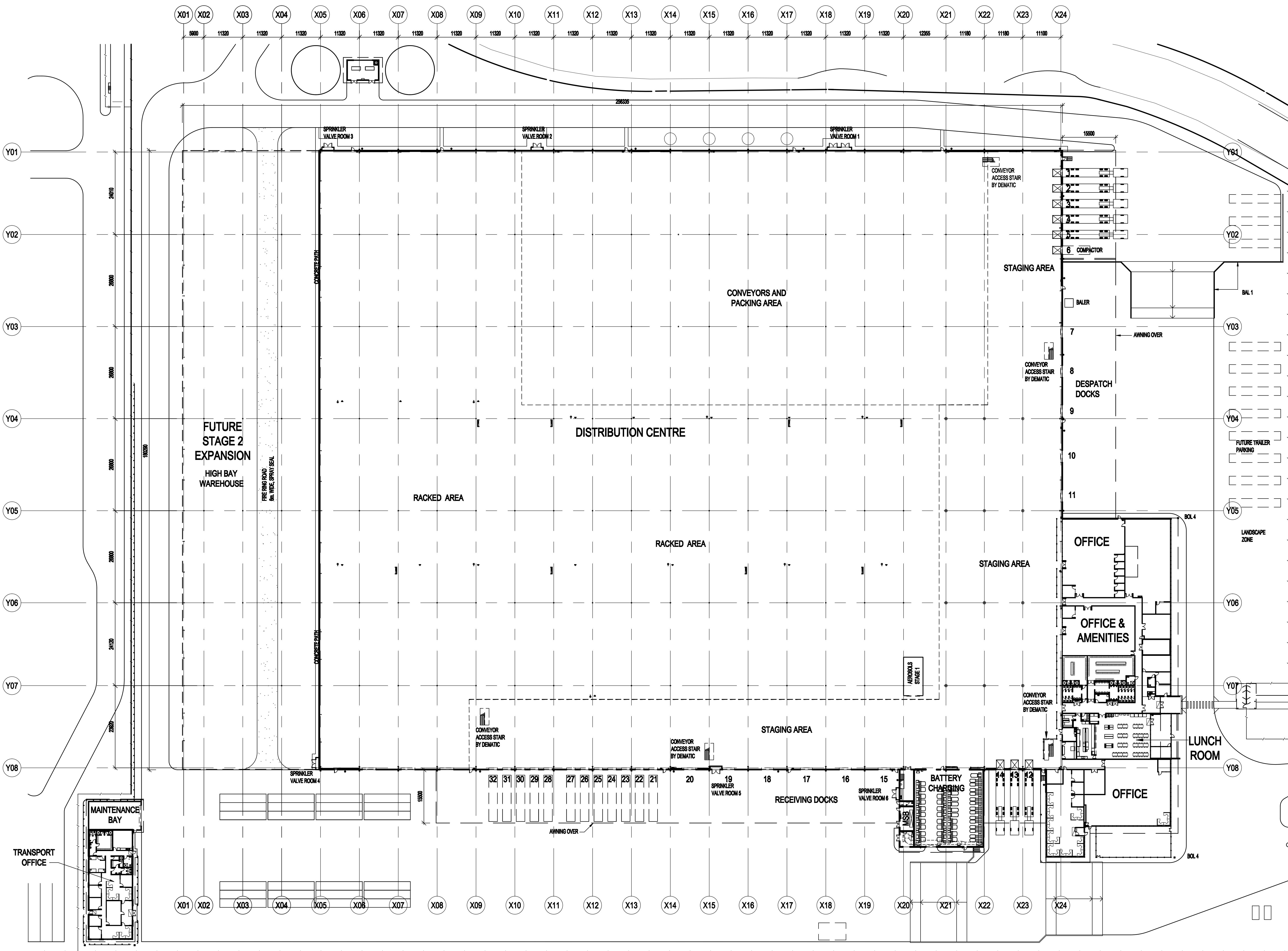
01 FLOOR PLAN
