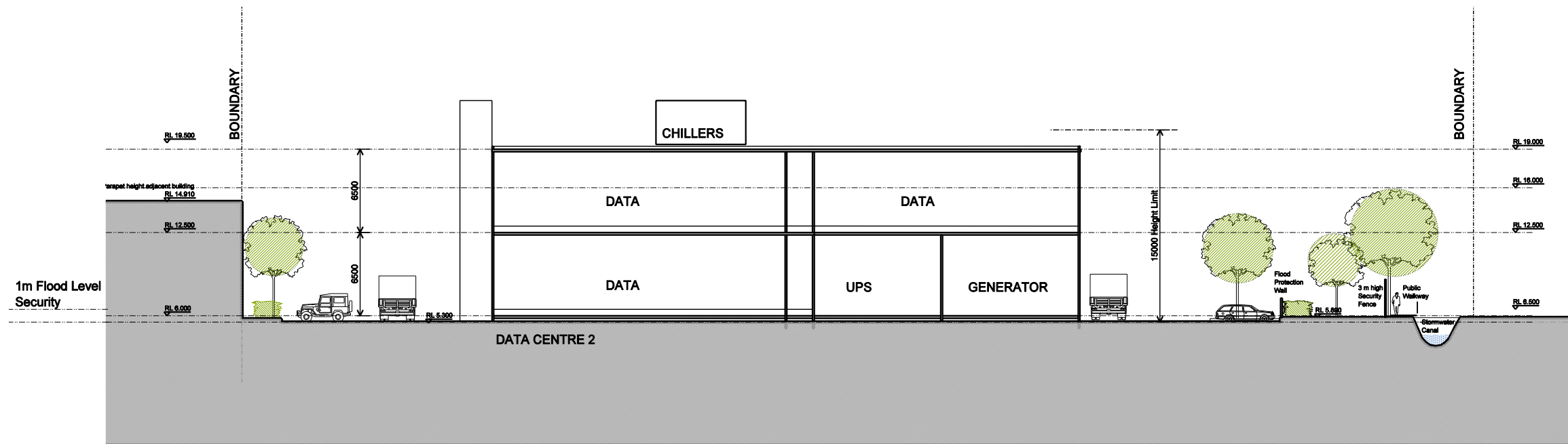
Section AA
