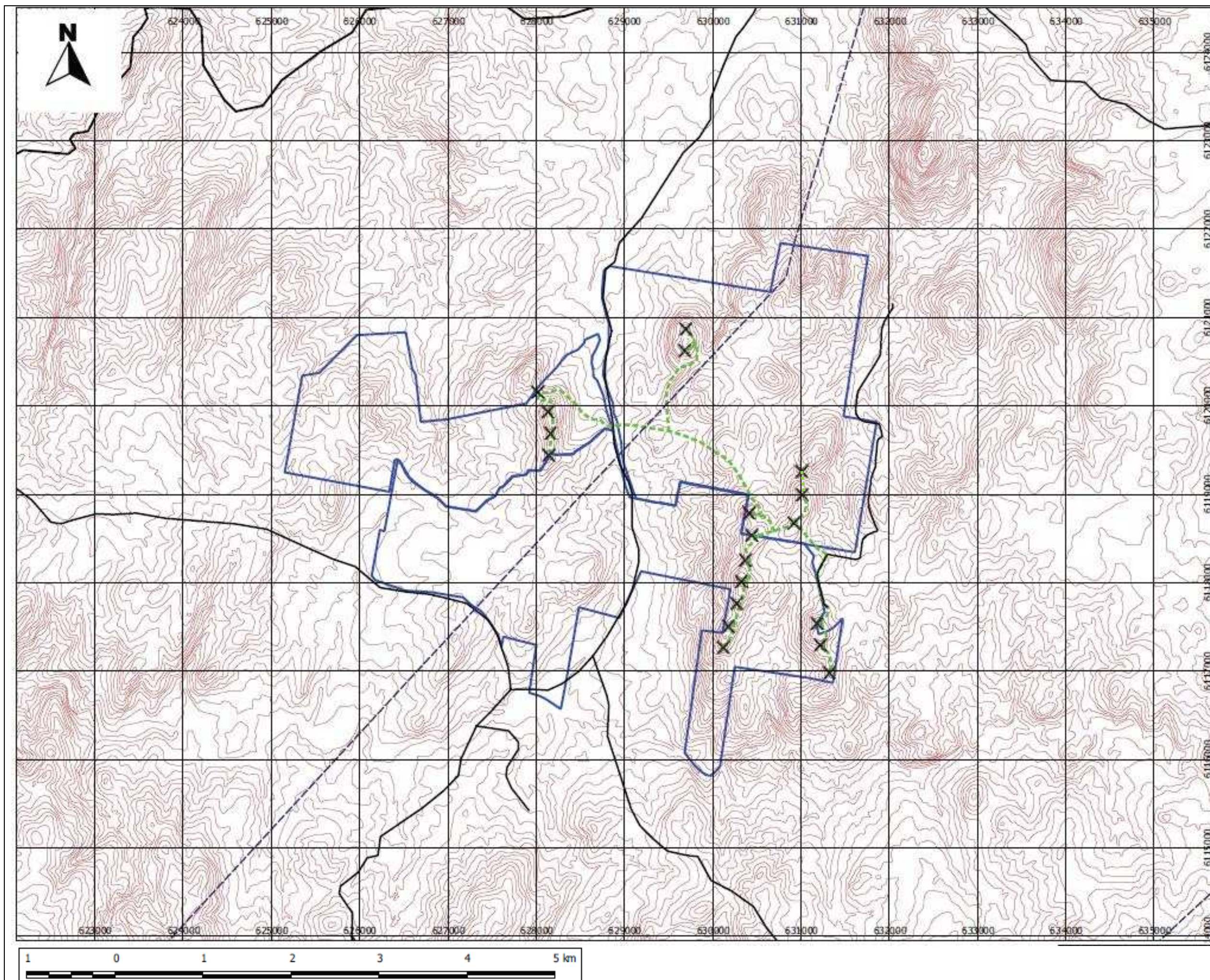
FIGURE 3: ADJUNGBILLY WIND FARM "ADJUNGBILLY CLUSTER"- PROPOSED TURBINE LOCATIONS
