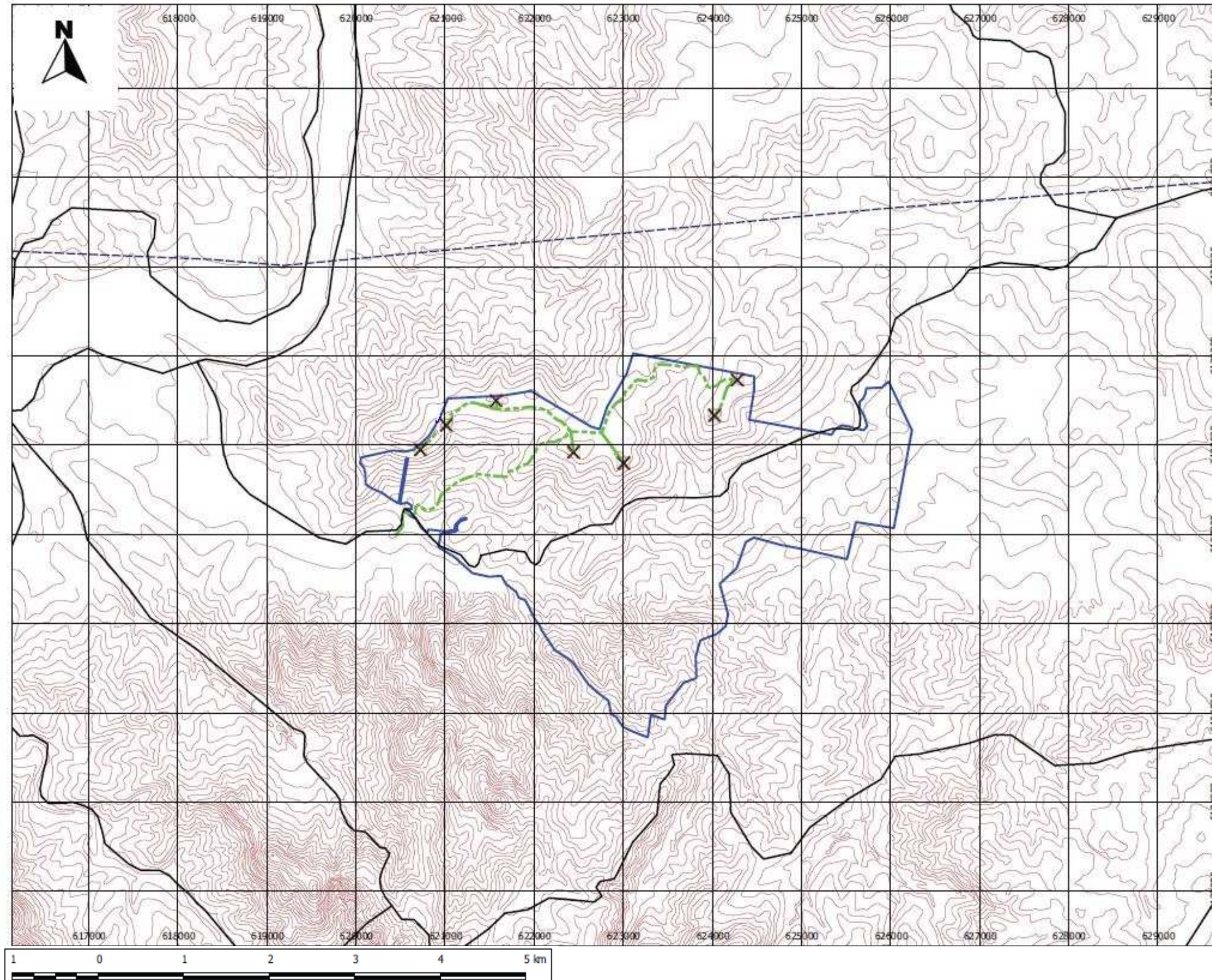
FIGURE 4: ADJUNGBILLY WIND FARM "STOCKDALE CLUSTER"- PROPOSED TURBINE LOCATIONS
