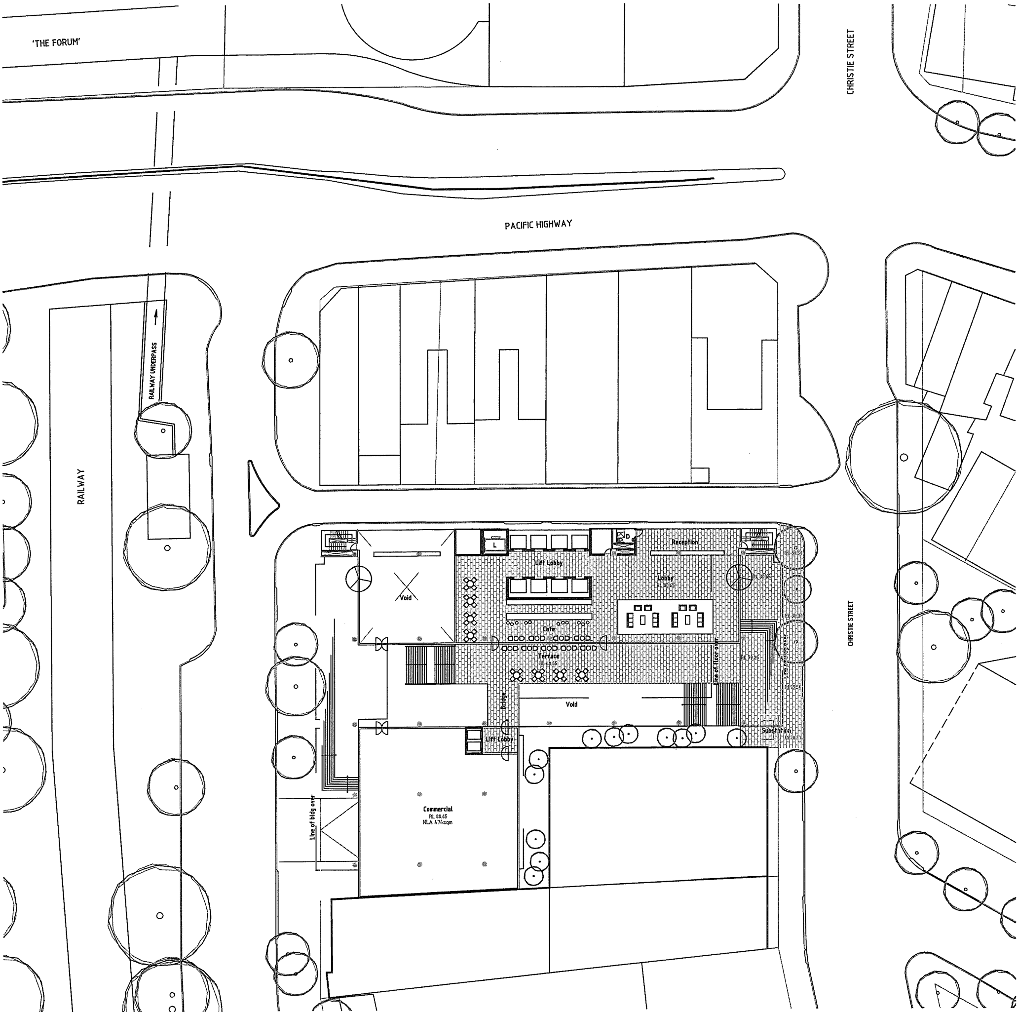
Christie Street, St Leonards Plan Ground 1:500
