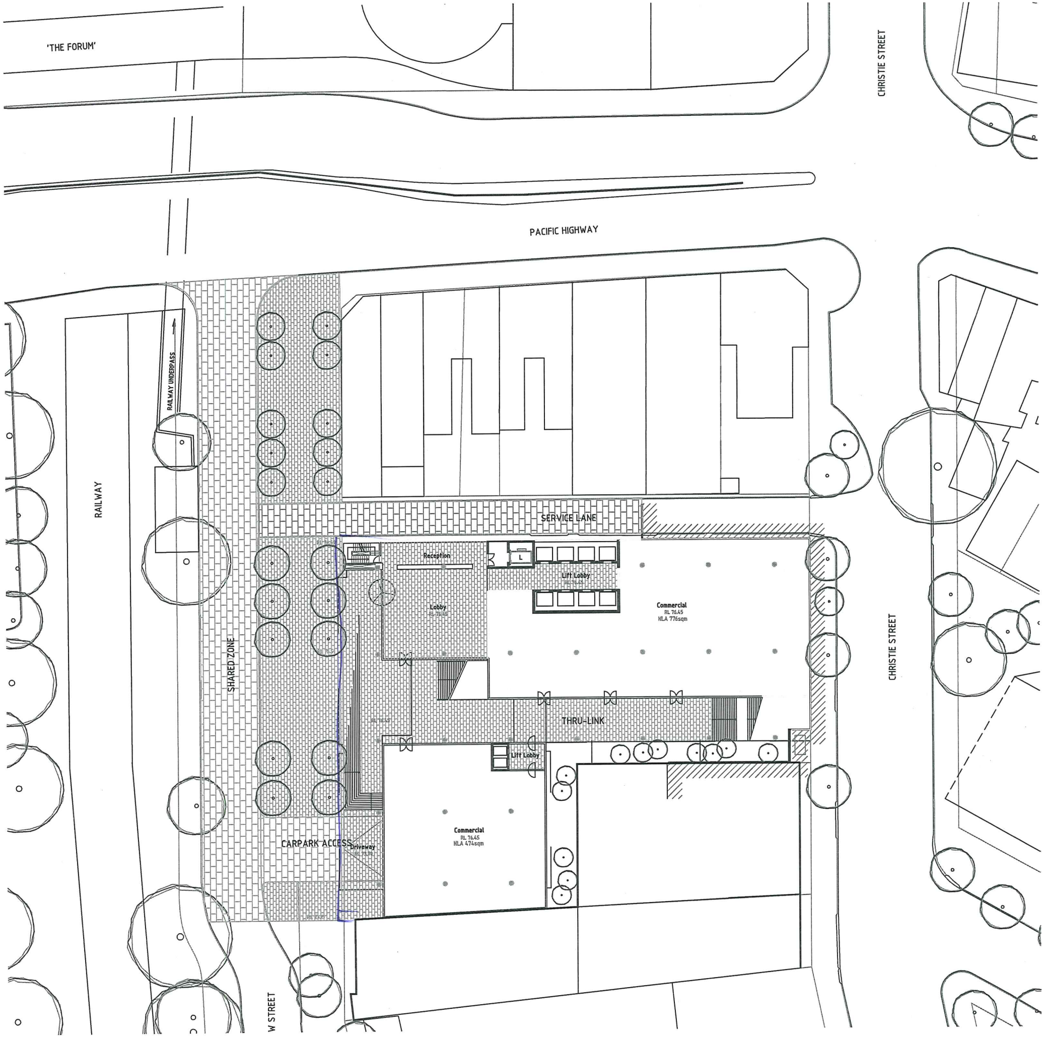
Christie Street, St Leonards Plan Lower Ground 1:500
