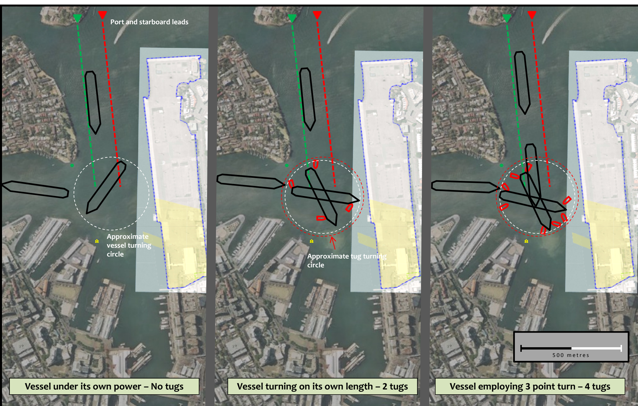
FIGURE 5 Impact of Landmark Building on turning circles for 300m vessel
