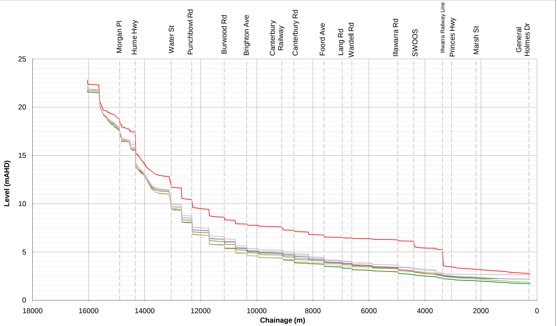
Figure 27 Cooks River Design Event Flood Profiles
