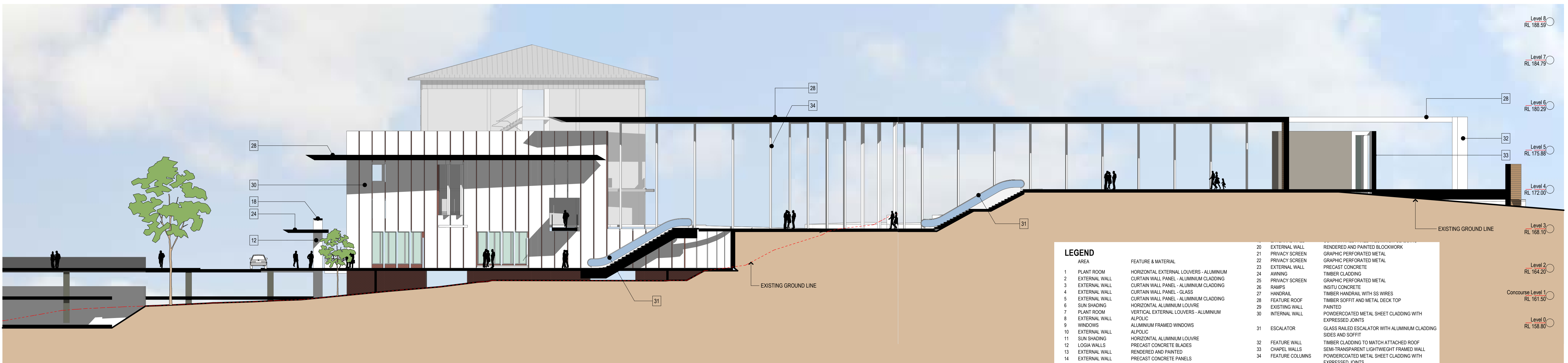
CONCOURSE SECTION
