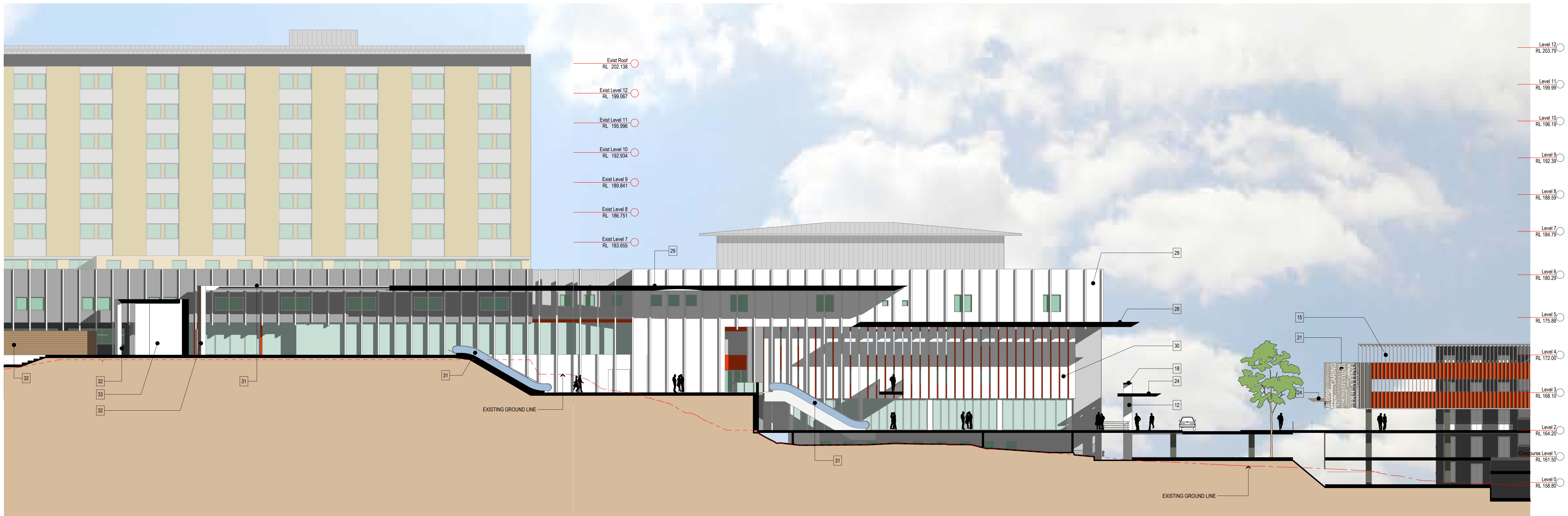
CONCOURSE SECTION
