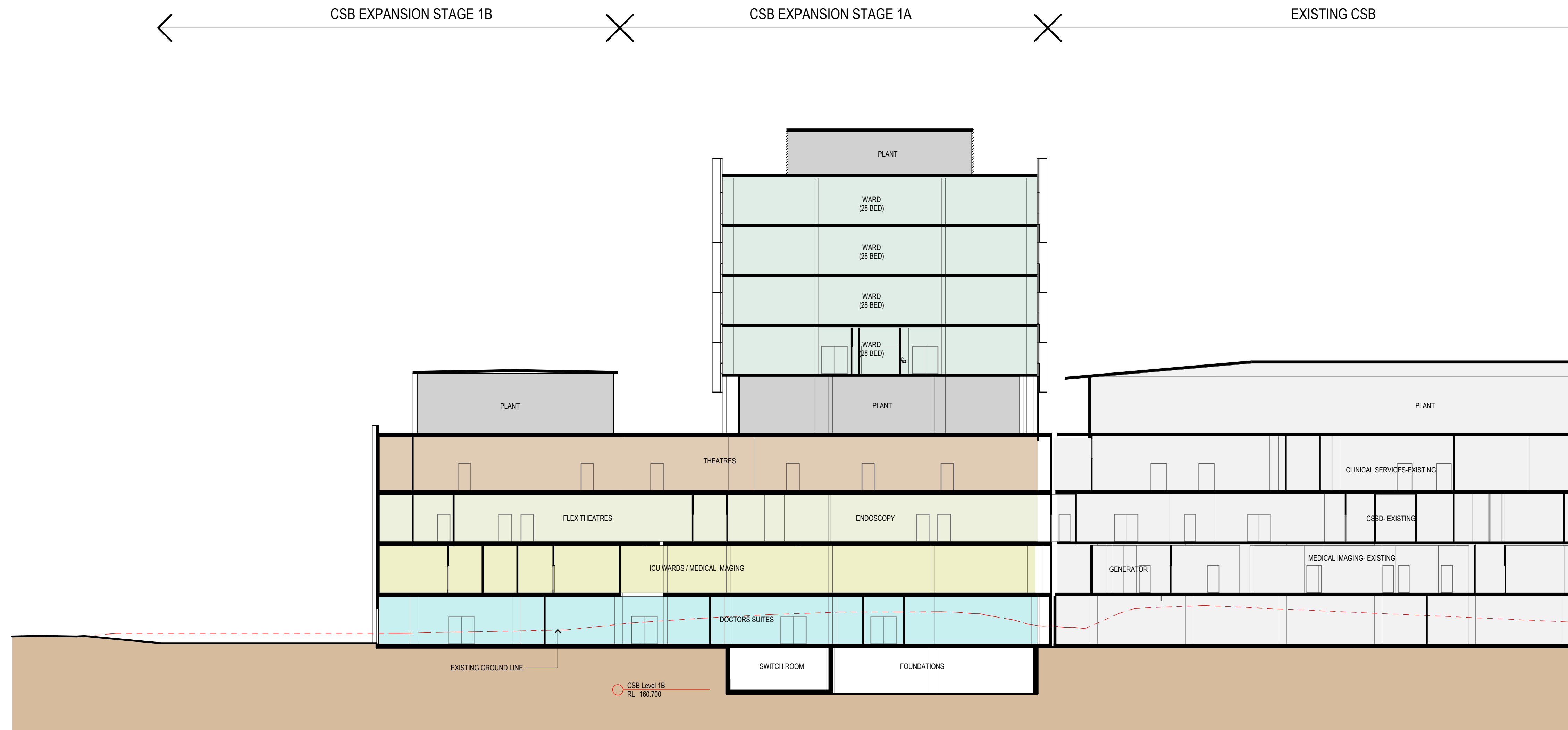
06 CSB SECTION SCALE 1:200
