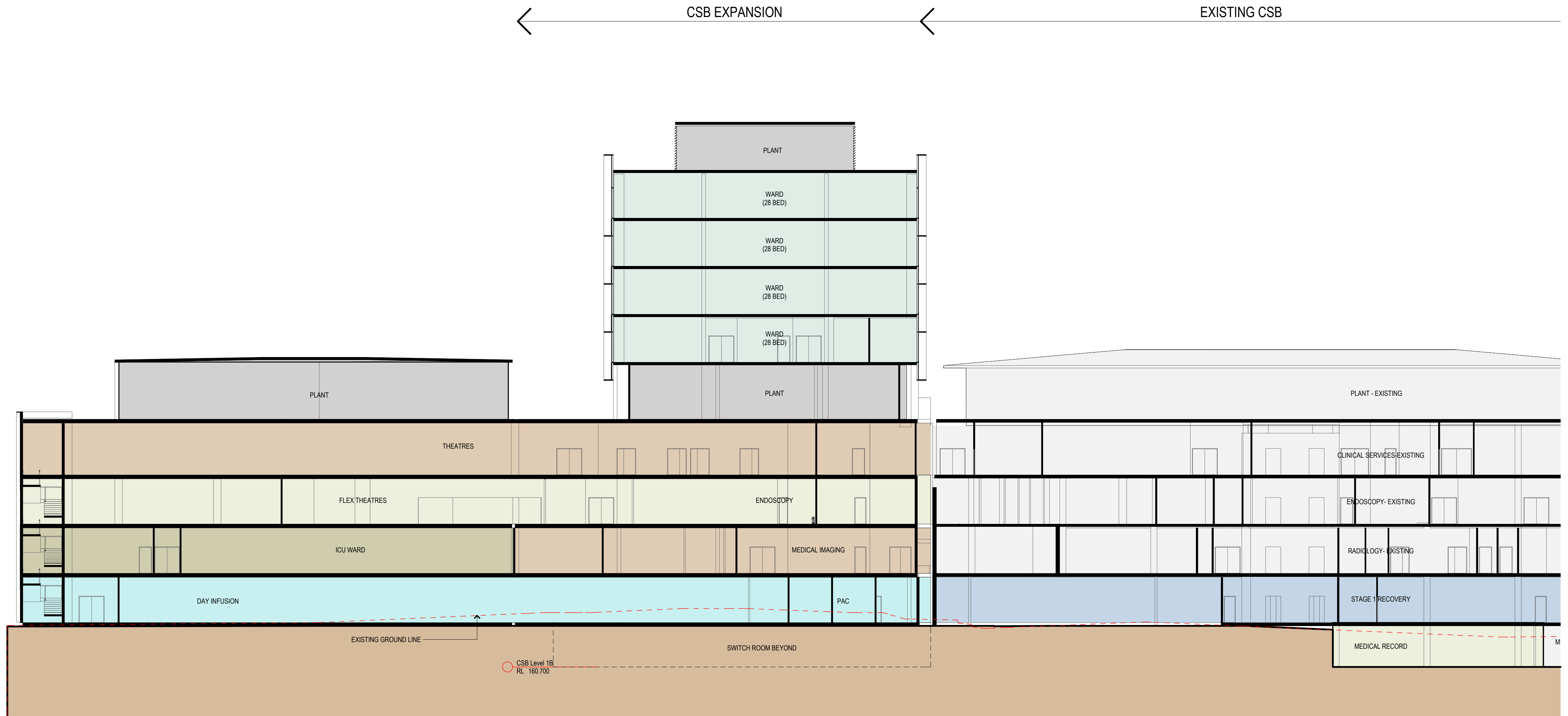
05 CSB SECTION SCALE 1:200
