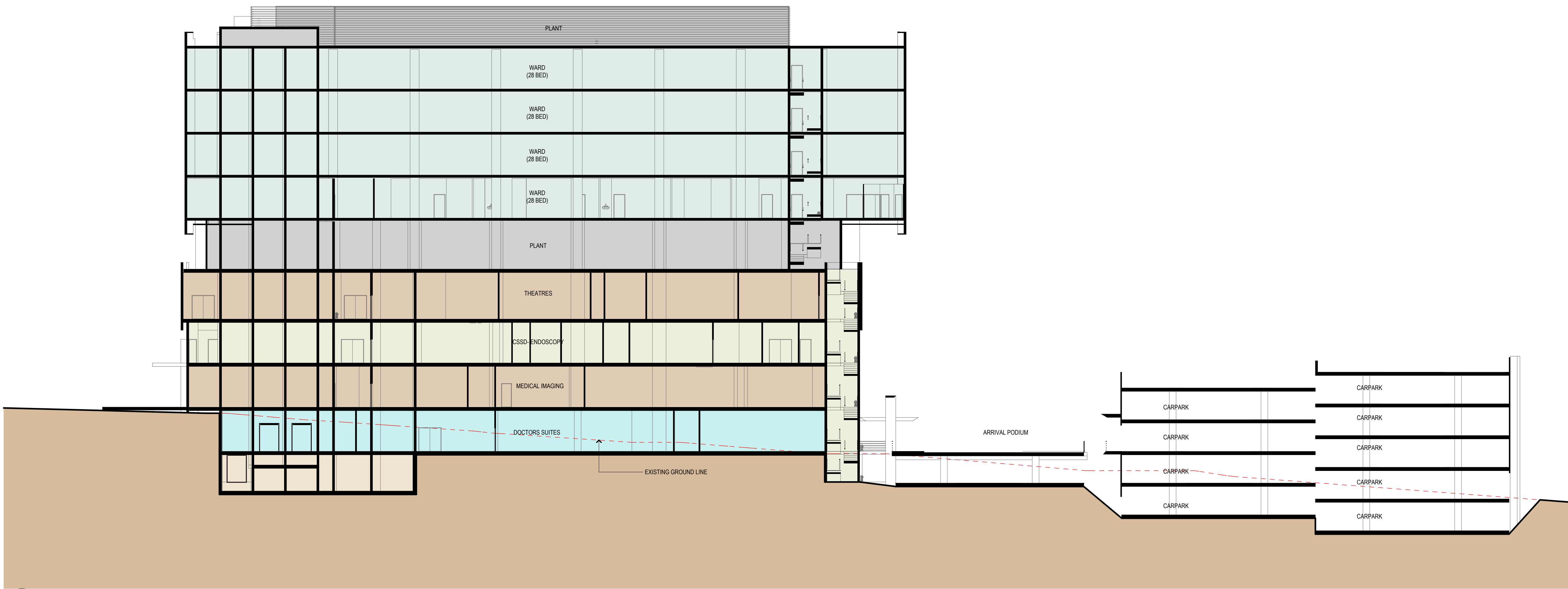
07 CSB SECTION SCALE 1:200
