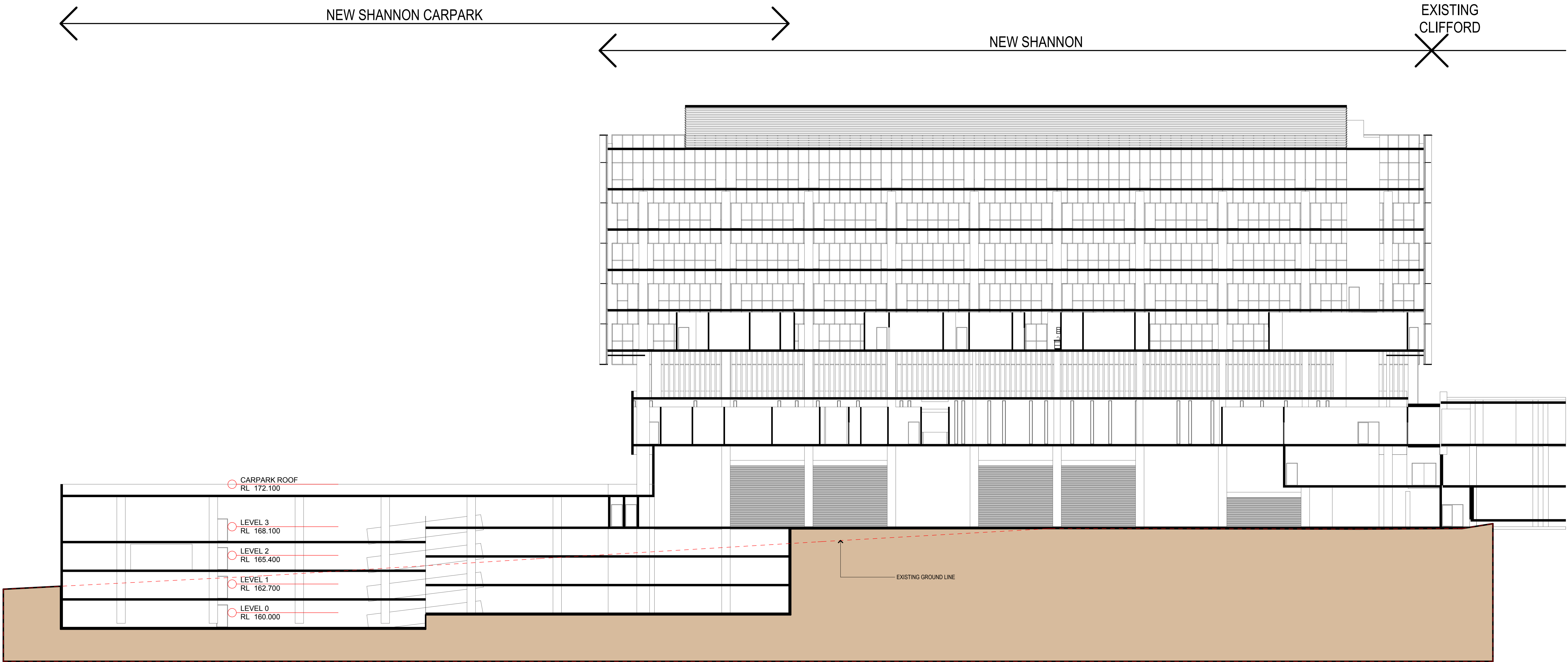
1 SHANNON SECTION SCALE 1:200
