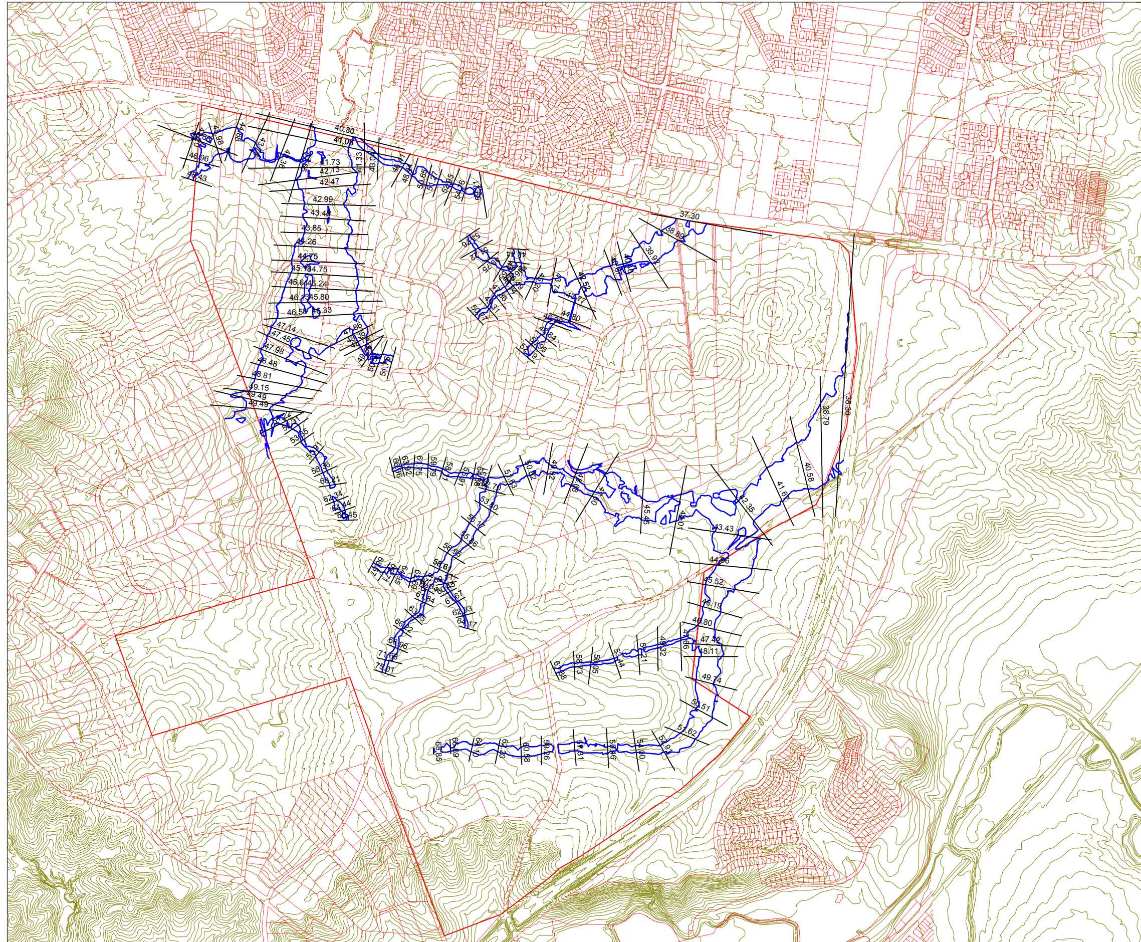
FIGURE B-2 100-year ARI Existing Conditions Flood Levels and Extents
