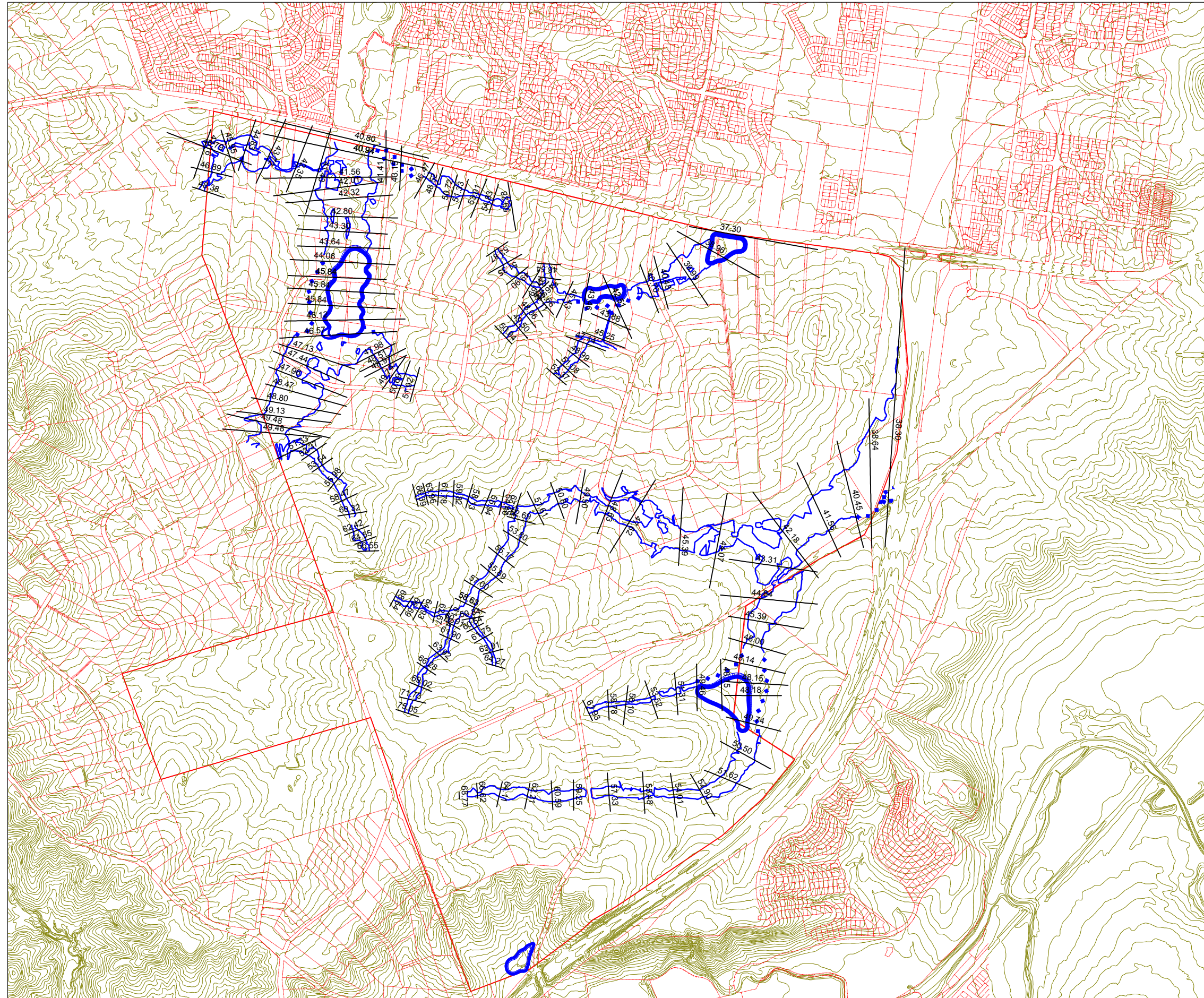
FIGURE B-6 20-year ARI Developed Conditions Flood Levels and Extents, with Mitigation
