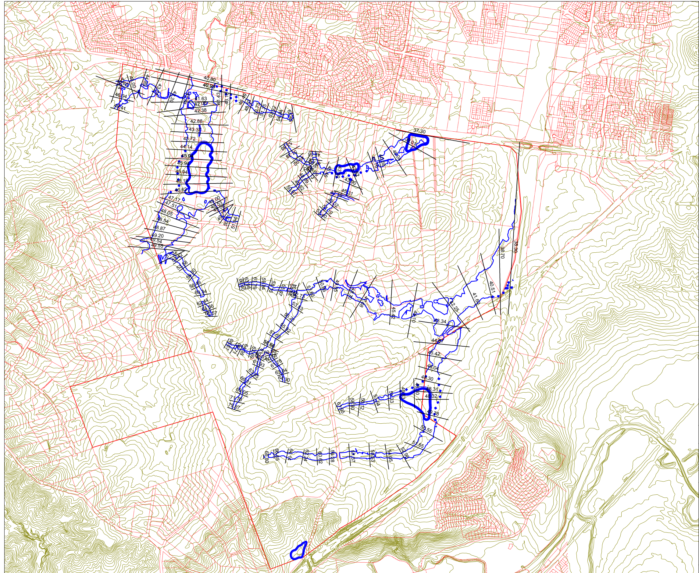
FIGURE B-5 50-year ARI Developed Conditions Flood Levels and Extents, with Mitigation
