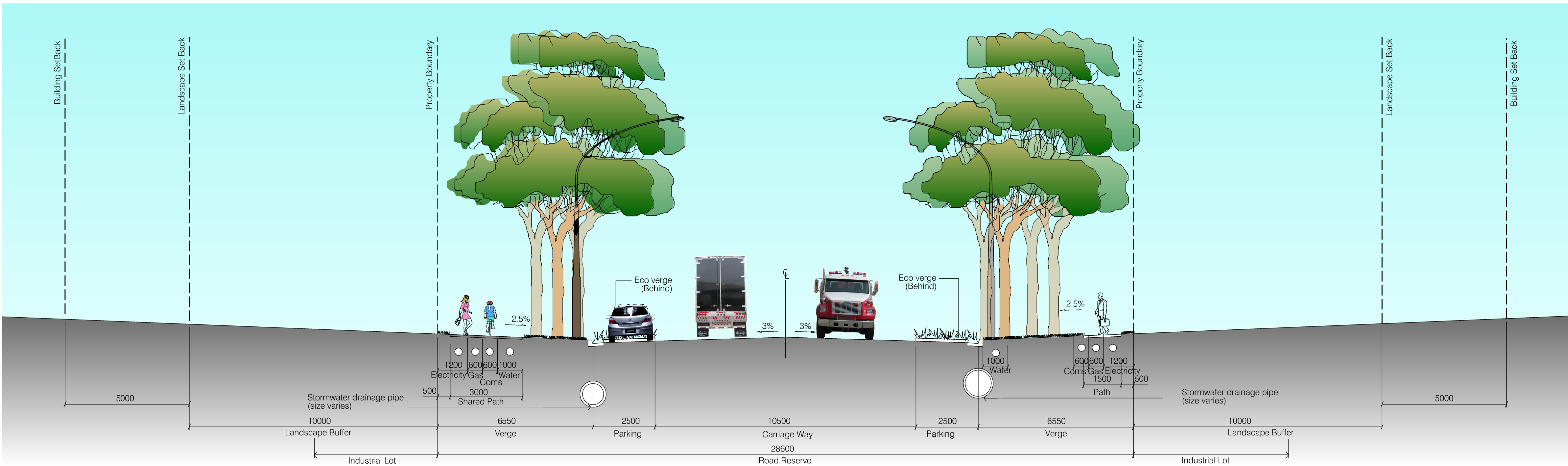
A ROAD 4 - ENTRY BOULEVARD Typical Section Garden Bed
