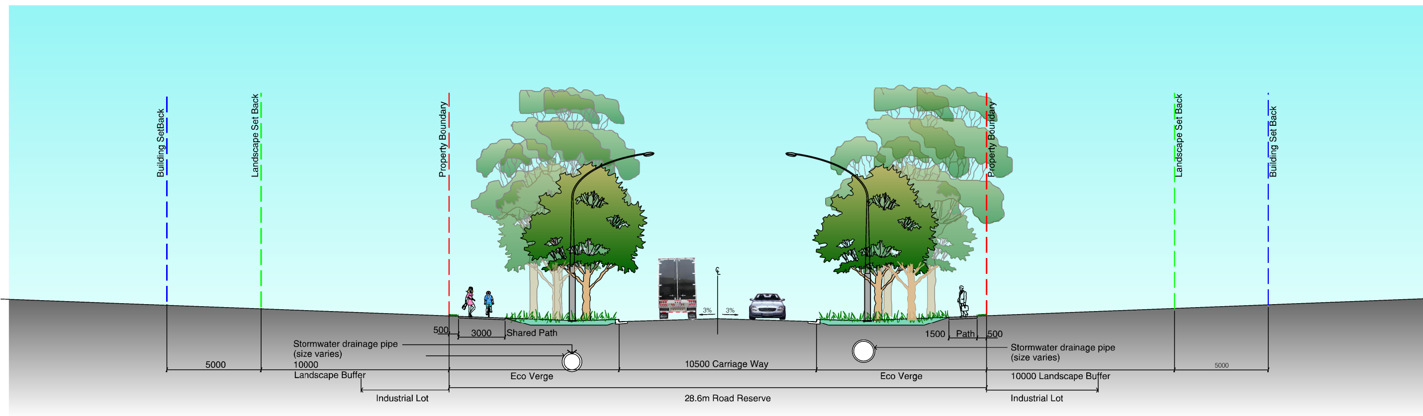
A ROAD 4 - ENTRY BOULEVARD Typical Section Rain Garden
