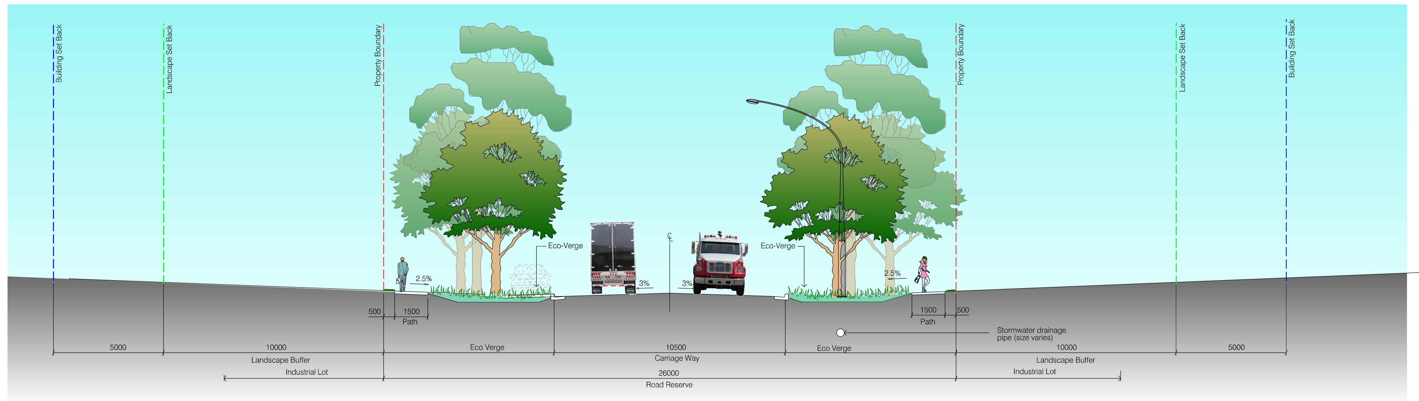
A ROAD 1 - COLLECTOR ROAD: Eco verge Typical Section through Eco verge - Note Local Roads Eco verge similar
