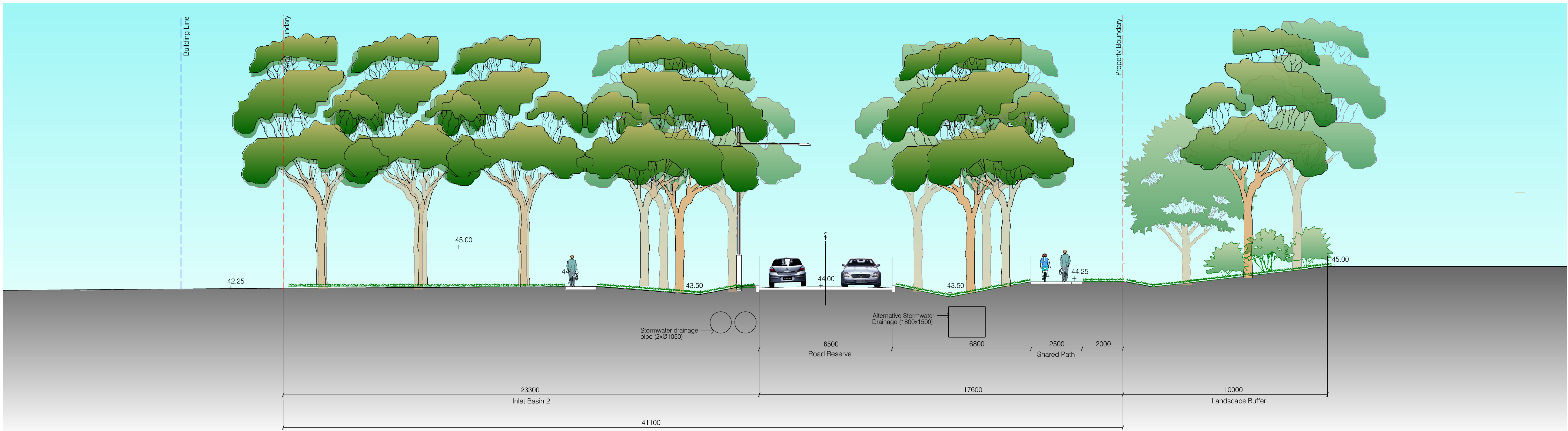
A LINK ROAD & INLET BASIN 2 Typical Section
