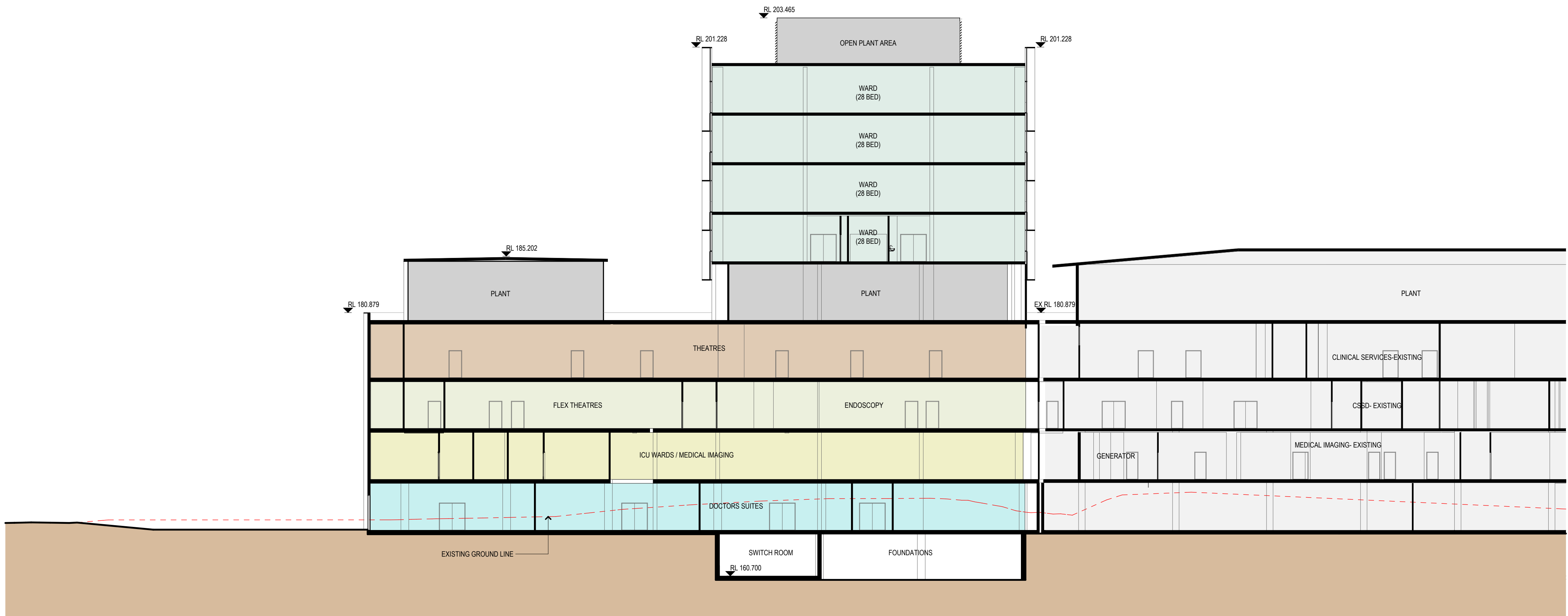
06 CSB SECTION SCALE 1:200
