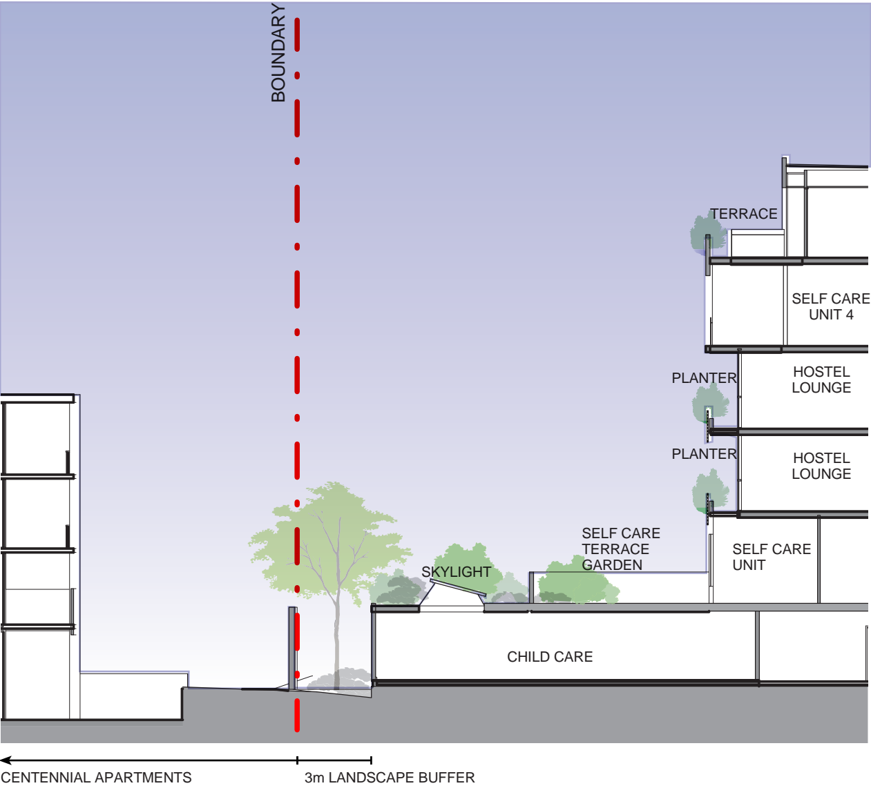
DETAIL SECTION - SECTION 3
