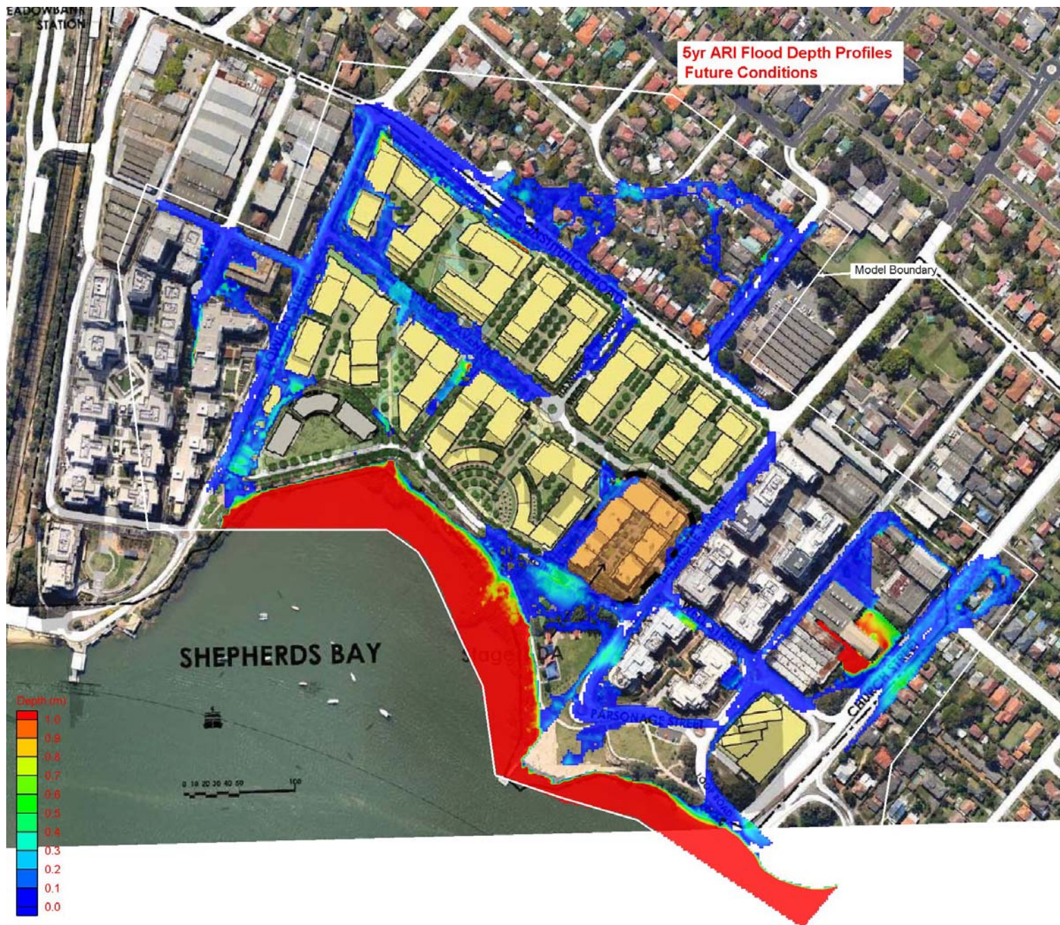
Figure 13 5 yr ARI Flood Levels – Future Conditions
