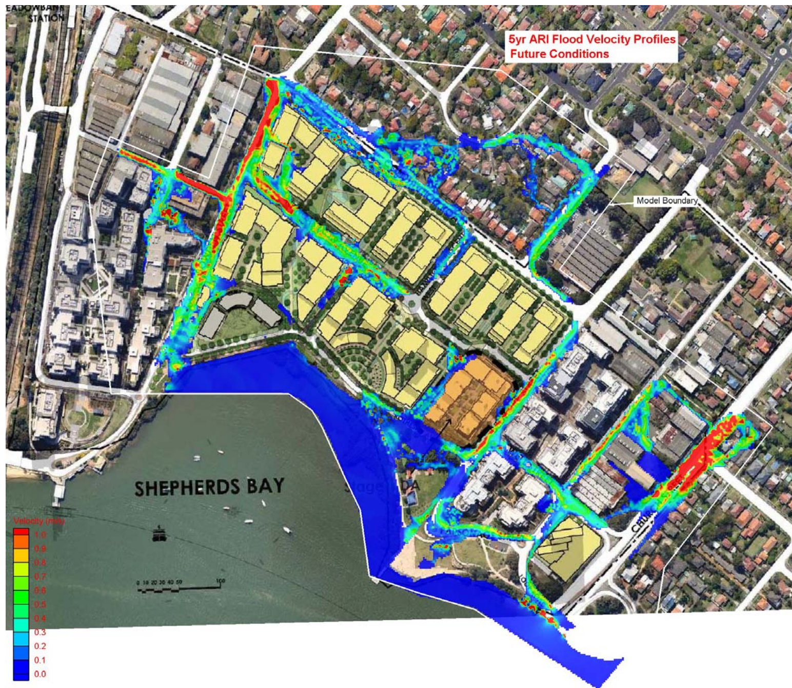
Figure 14 5 yr ARI Flood Velocities – Future Conditions
