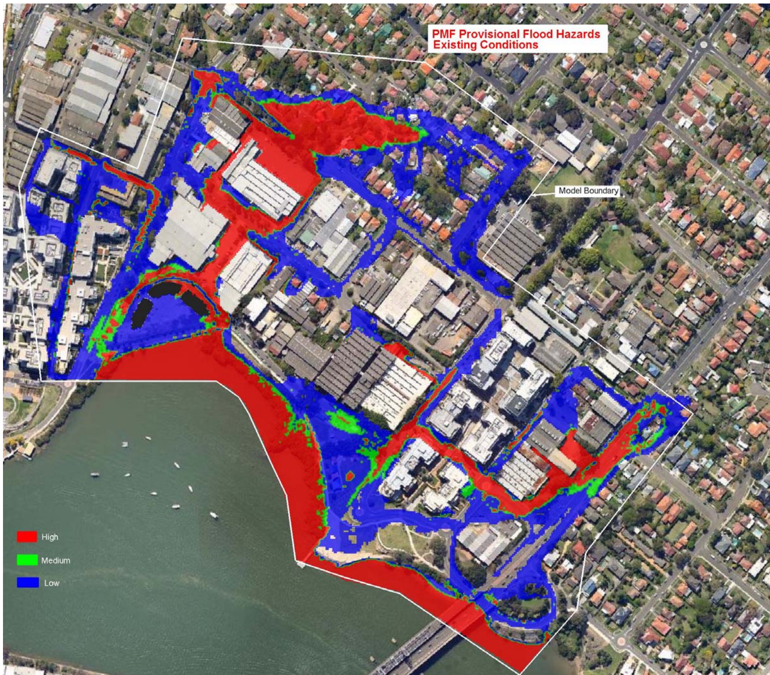
Figure 12 PMF Flood Hazard – Existing Conditions
