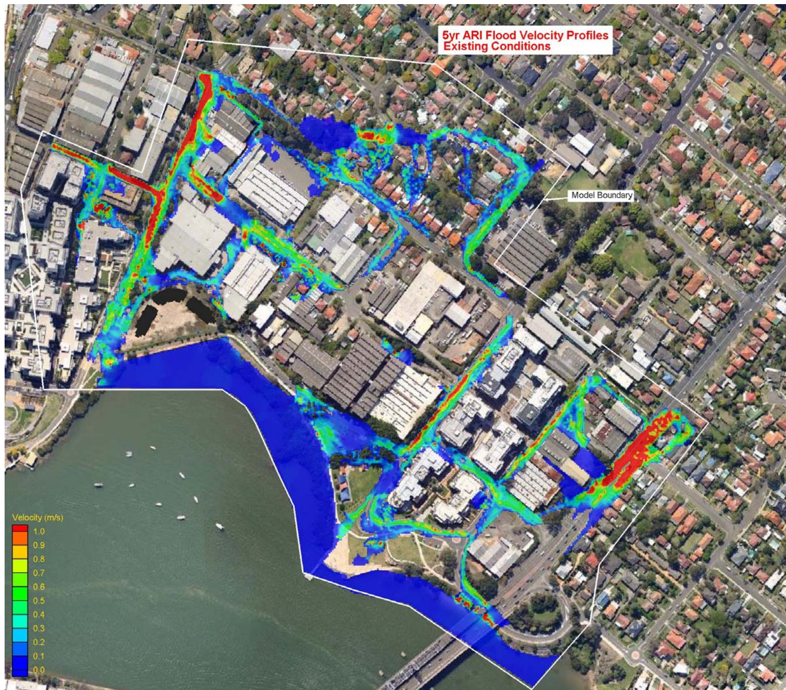
Figure 2 5 yr ARI Flood Velocities – Existing Conditions
